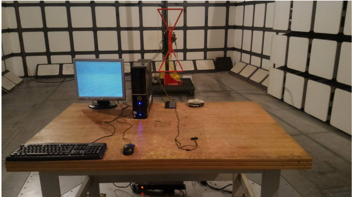
Radiated Emissions – Front View (Below 1 GHz)
