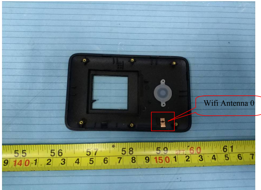
EUT – Wifi Antenna 0 View
