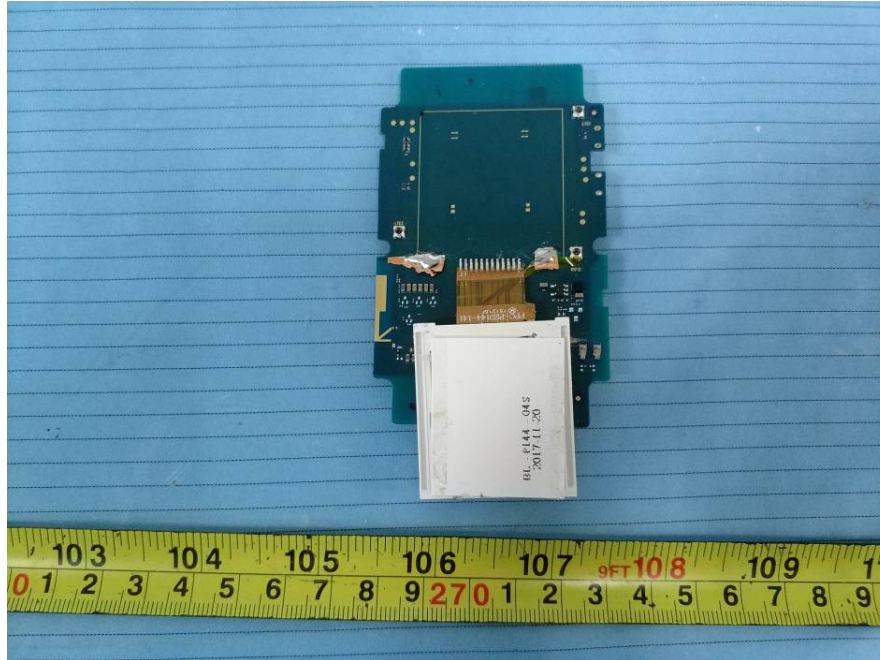
EUT – PCB Top Shielding off View 2
