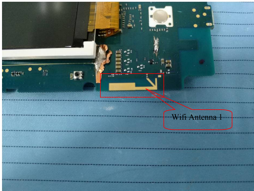
EUT – Wifi Antenna 1 View
