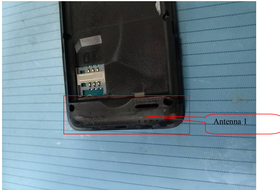
EUT – 2G & 3G & 4G Antenna 1 View (Main Antenna)
