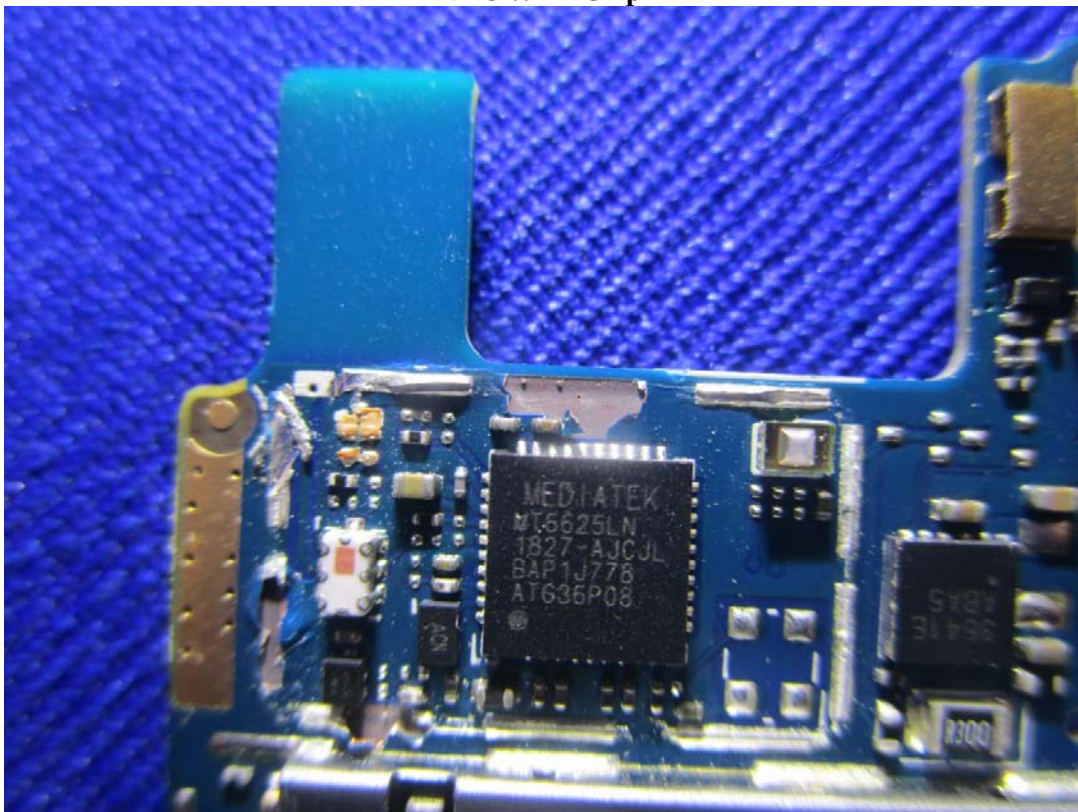
BT&WIFI Chip
