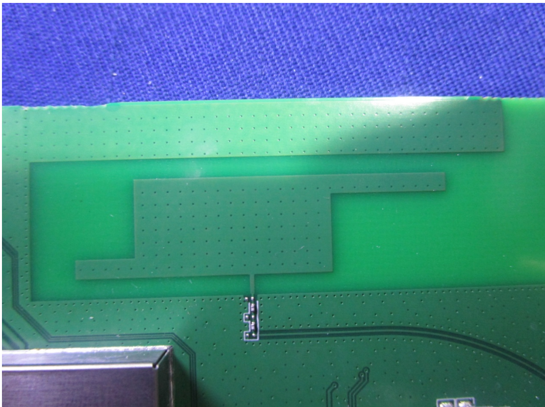
WCDMA &LTE Main Antenna View
