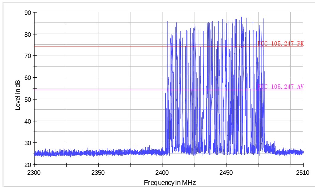
Copy of FCC Electric Field Strength 1-18GHz
