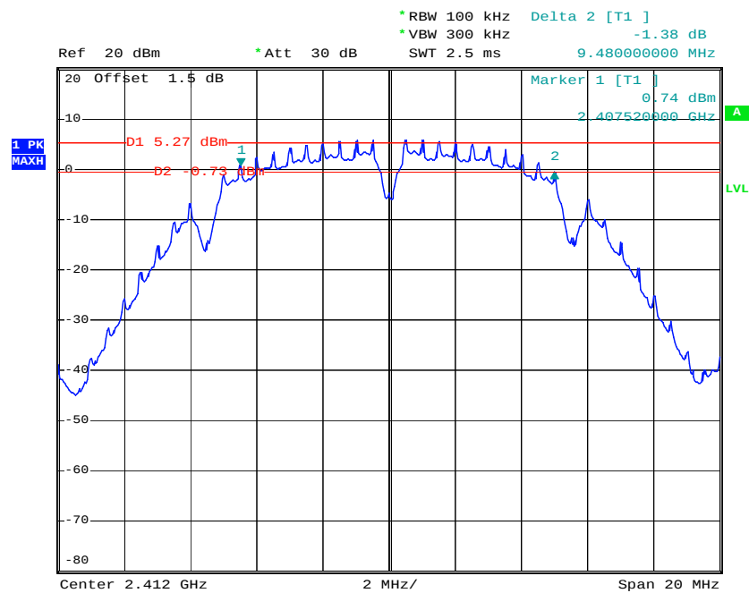
Mode 1 : 6 dB Bandwidth Plot on 802.11b Channel 01
