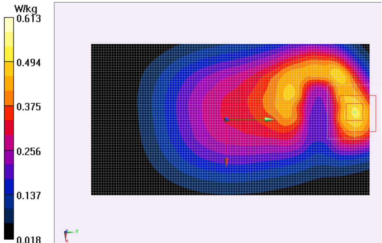
Fig.2 8350 MHz CH190
