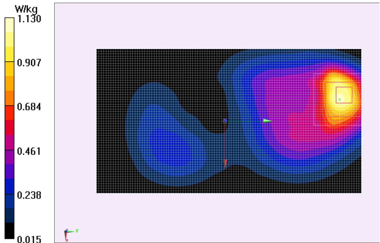
Fig.2 1900 MHz CH661
