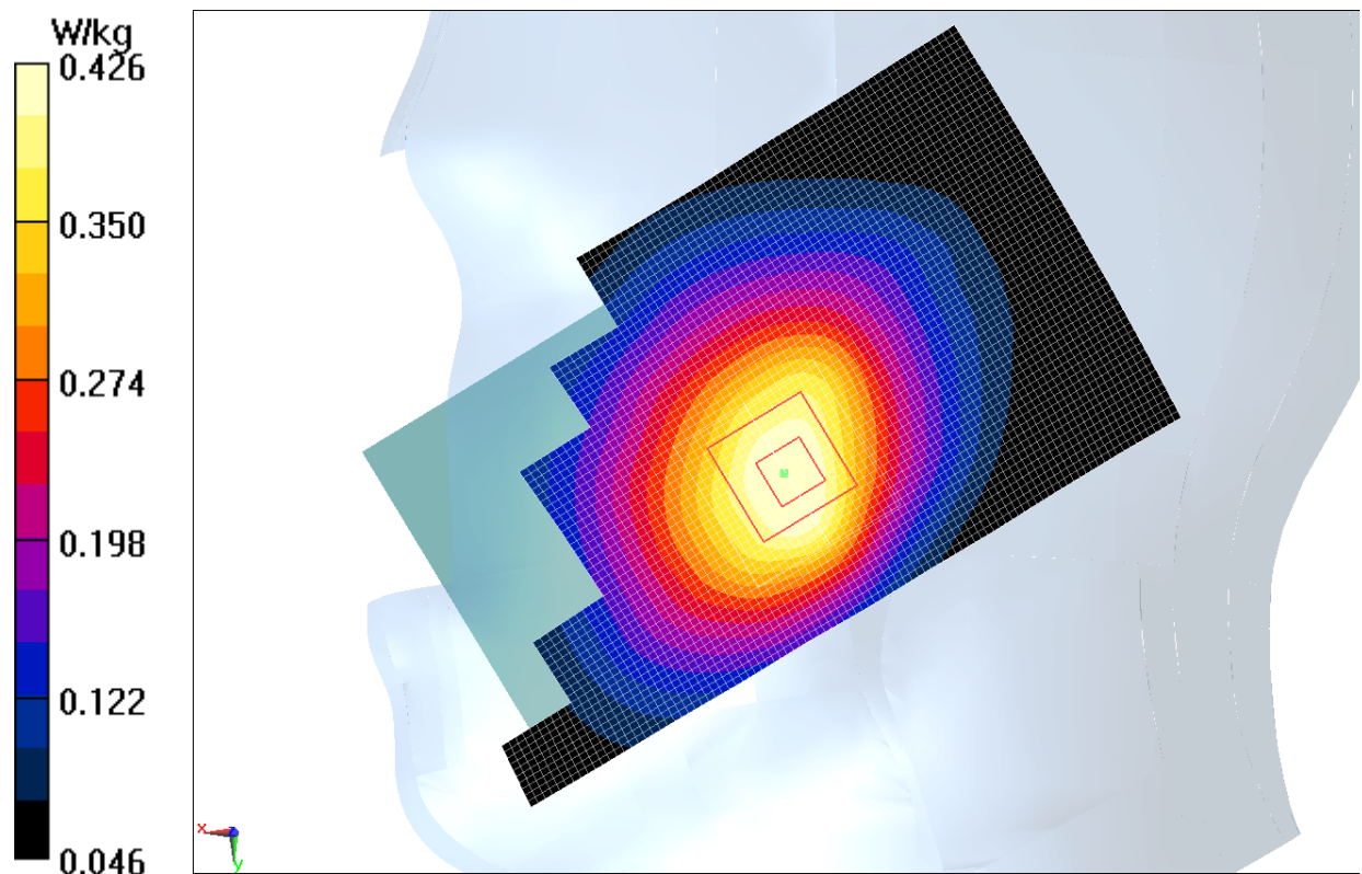
Fig.1 850 MHz CH251
