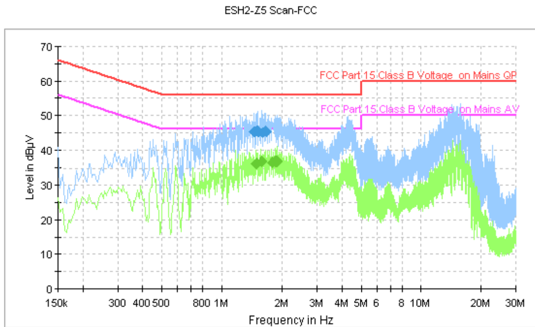
Fig.31 AC Powerline Conducted Emission (Traffic, AE1)
