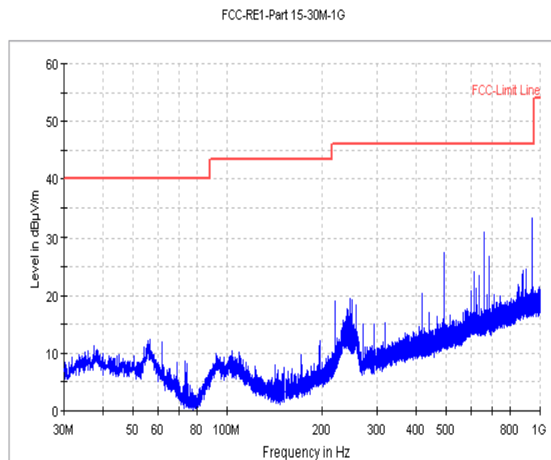
Fig.24 Radiated Spurious Emission (Ch19, 30 MHz-1 GHz)
