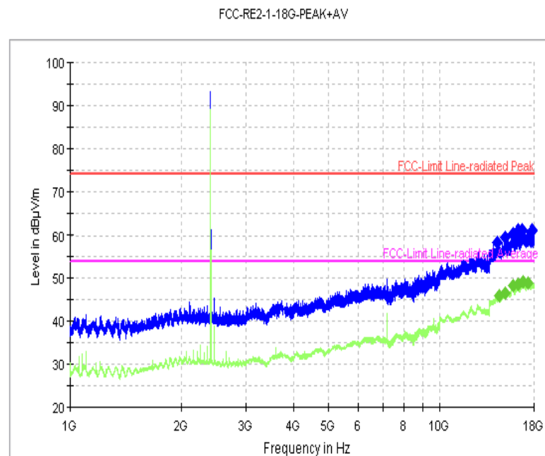
Fig. 51 Radiated Spurious Emission (GFSK, Ch0, 1 GHz ~18 GHz)
