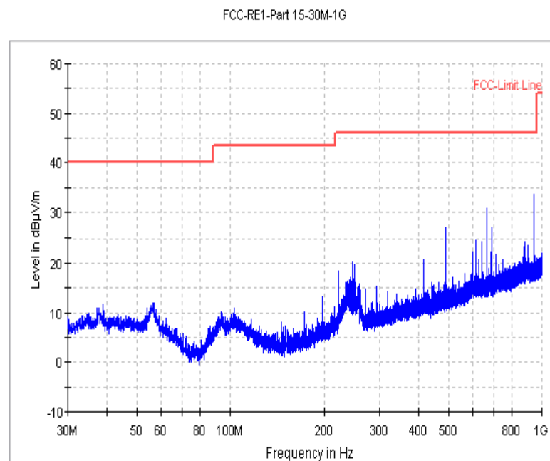
Fig. 52 Radiated Spurious Emission (GFSK, Ch39, 30 MHz ~1 GHz)
