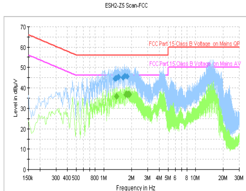
Fig. 99 AC Power line Conducted Emission (Traffic, AE1)
