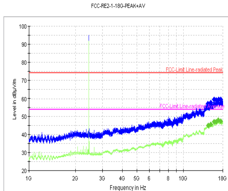
Fig. 69 Radiated Spurious Emission (8DPSK, Ch39, 1 GHz ~18 GHz)
