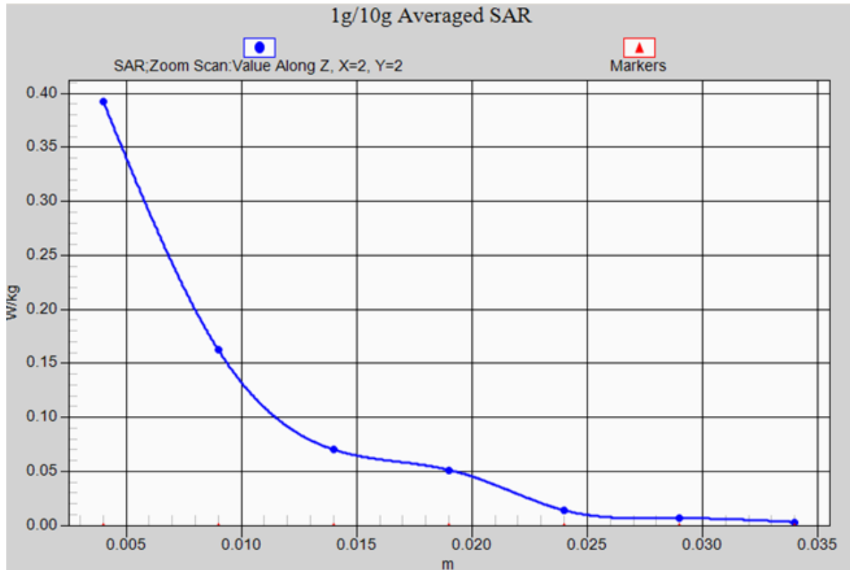
WiFi 802.11b RIGHT/CHEEK-High_ axis scan
