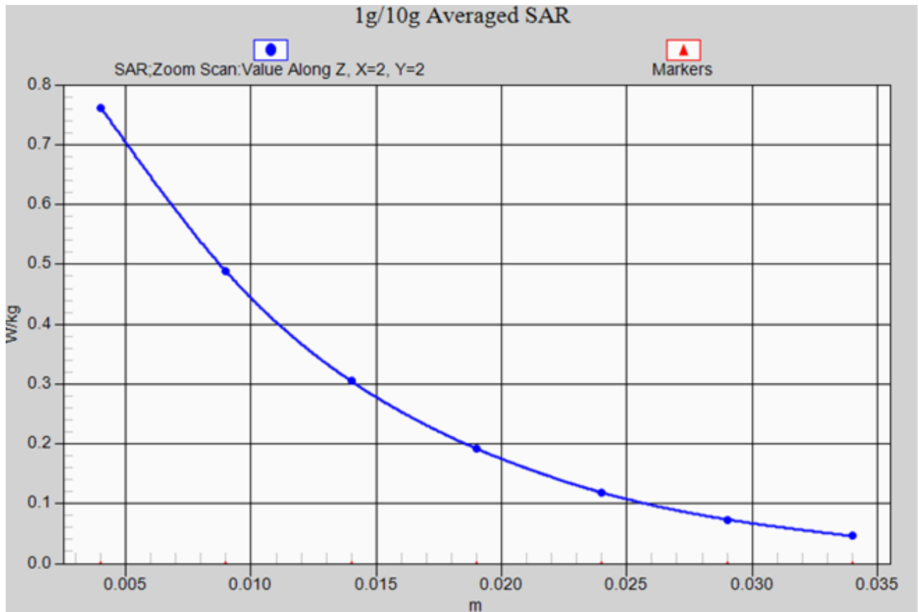
PCS1900 LEFT/CHEEK-Low_axis scan
