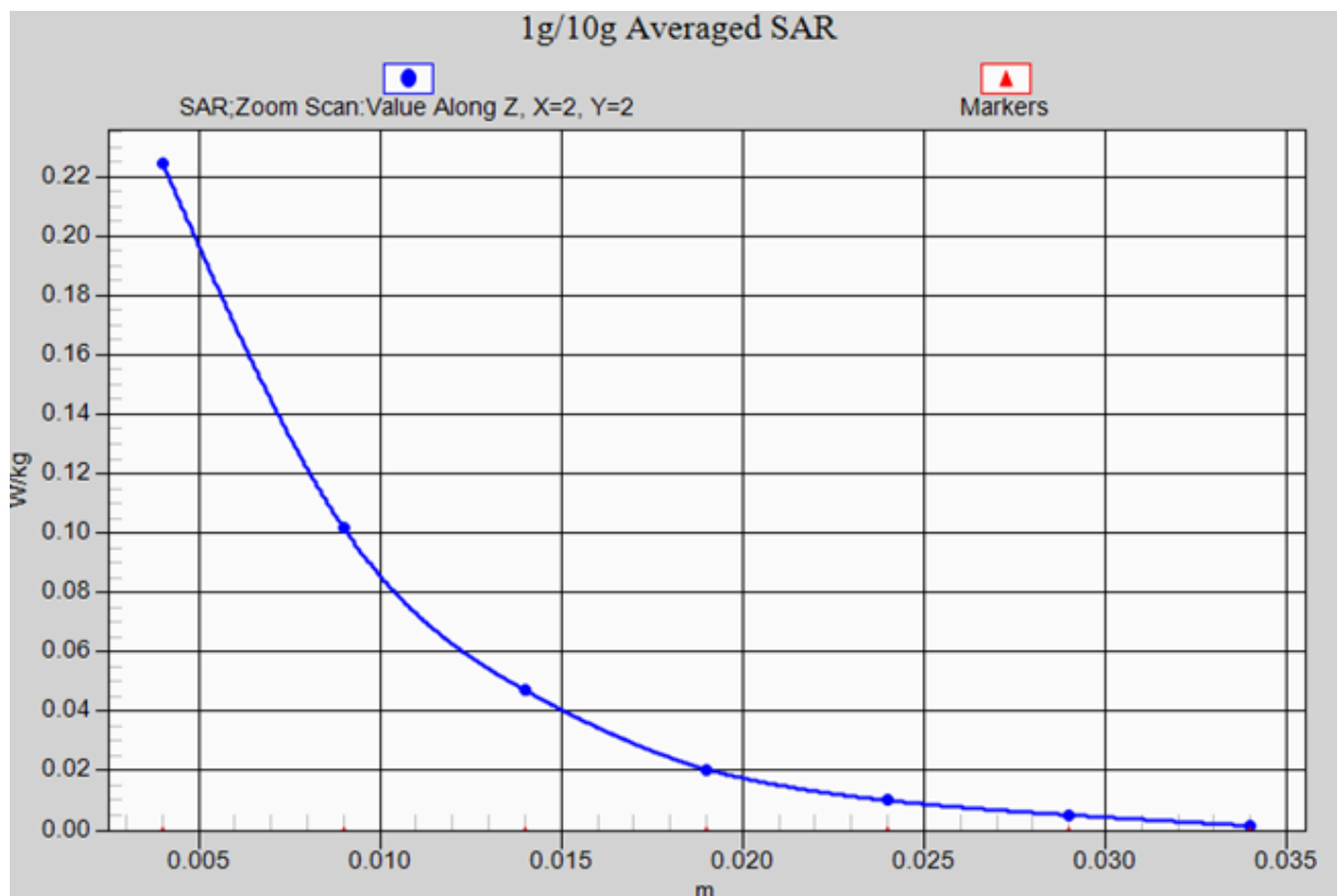
WiFi 802.11b/Back side-High_ axis scan
