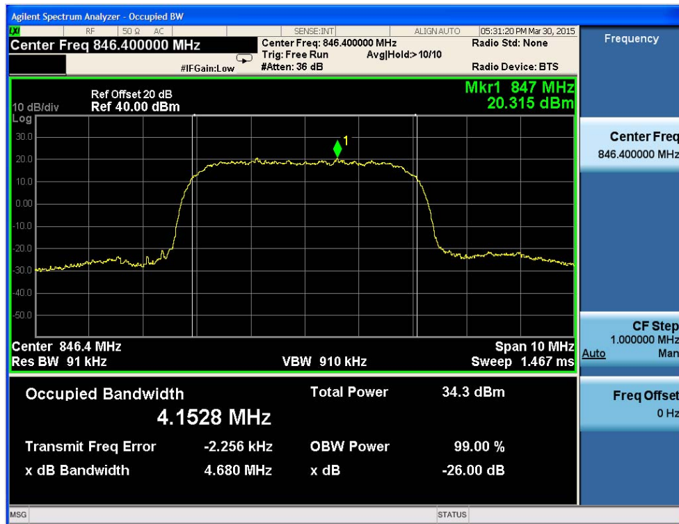
Fig.9 WCDMA Band V-CH4232 Occupied Bandwidth
