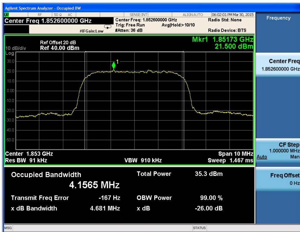
Fig.16 WCDMA Band II-CH9263 Occupied Bandwidth
