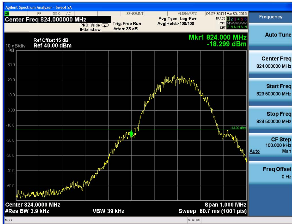
Fig.25 GSM850-CH128 Band Edge Compliance
