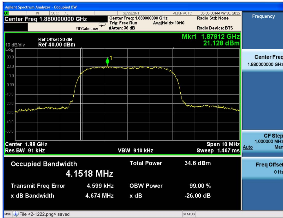
Fig.17 WCDMA Band II-CH9400 Occupied Bandwidth
