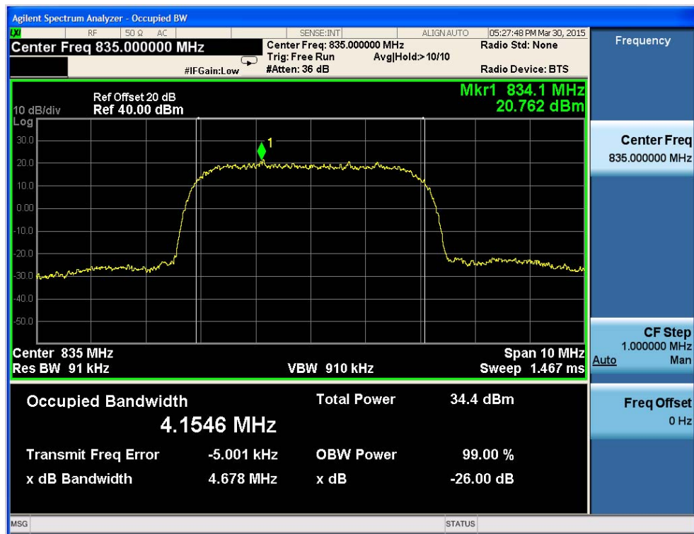
Fig.11 WCDMA Band V-CH4175 Occupied Bandwidth (HSDPA Subtest 1)
