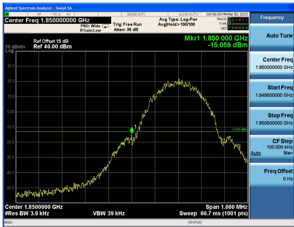
Fig.27 GSM1900-CH512 Band Edge Compliance
