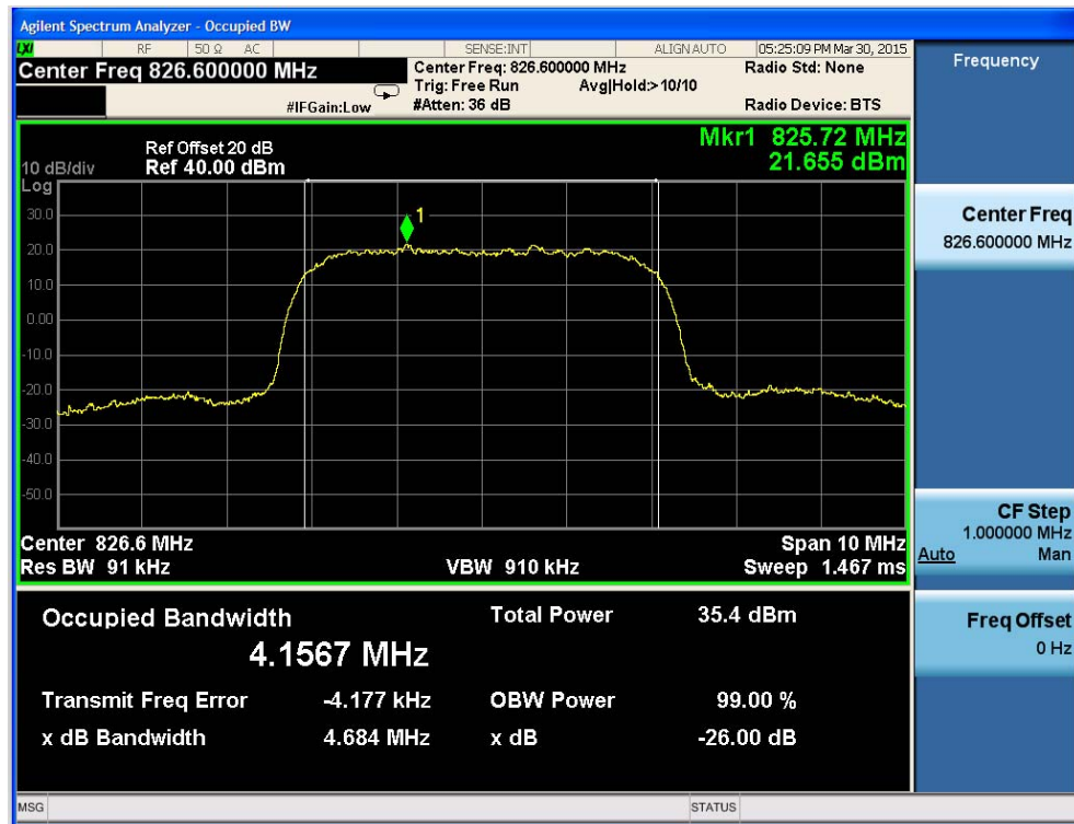
Fig.7 WCDMA Band V-CH4133 Occupied Bandwidth
