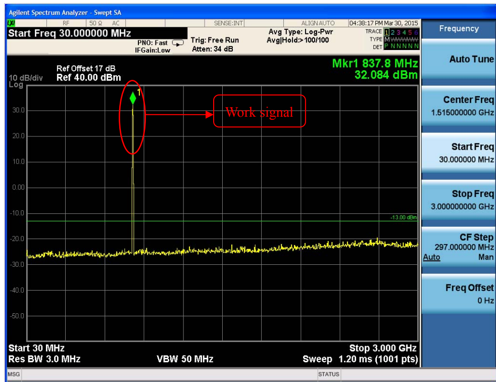
Fig.41 GSM850 on Channel 189 30MHz~3GHz
