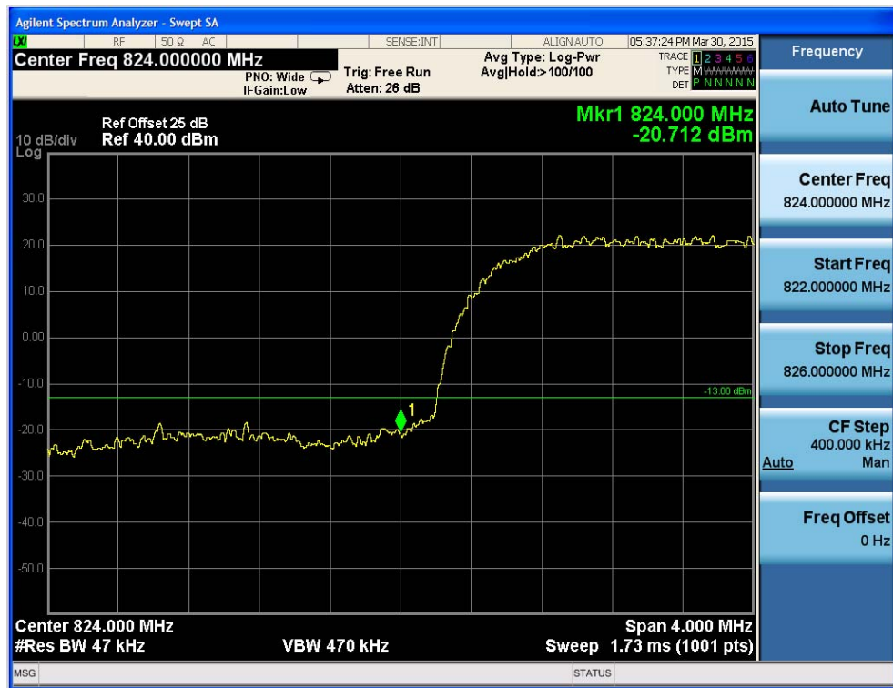
Fig.29 WCDMA Band V-CH4133 Band Edge Compliance
