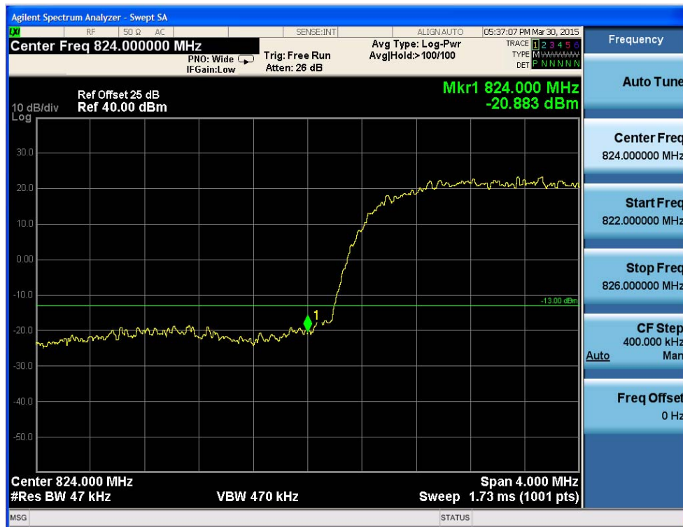
Fig.33 WCDMA Band V-CH4133 Band Edge Compliance HSUPA Subtest 5
