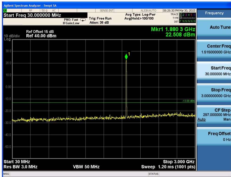
Fig.47 WCDMA Band II Channel 9400 30MHz~3GHz
