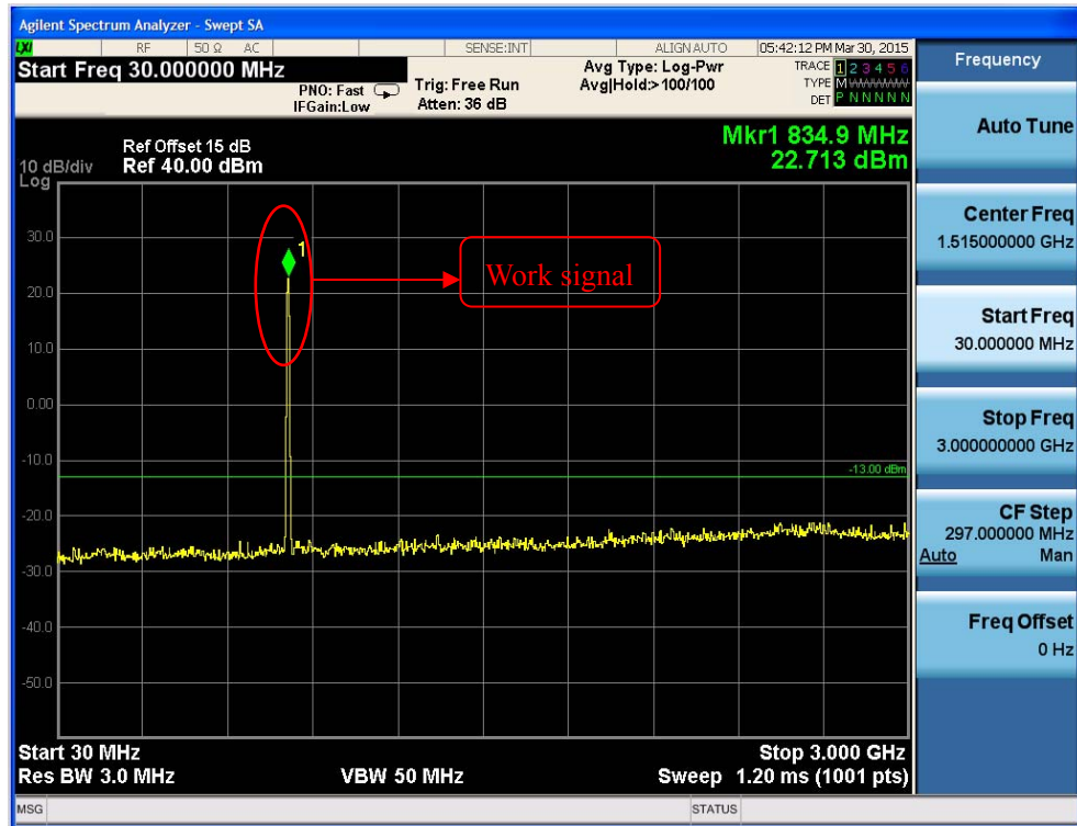
Fig.45 WCDMA Band V on Channel 4175 30MHz~3GHz
