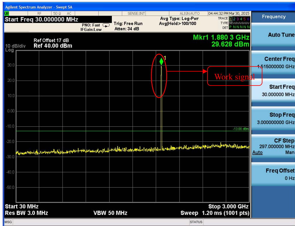
Fig.43 GSM1900 on Channel 661 30MHz~3GHz
