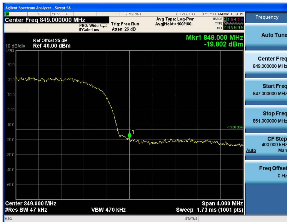
Fig.34 WCDMA Band V-CH4232 Band Edge Compliance HSUPA Subtest 5
