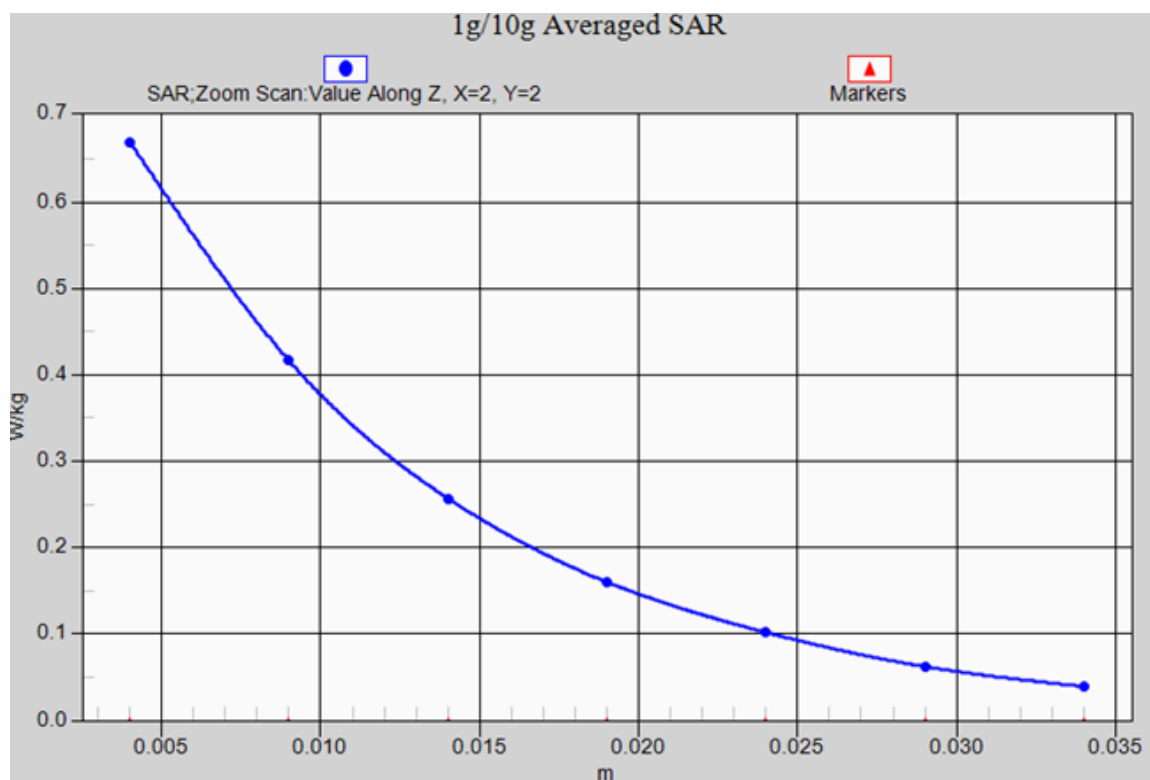
WCDMA Band II LEFT/CHEEK-Low_ axis scan
