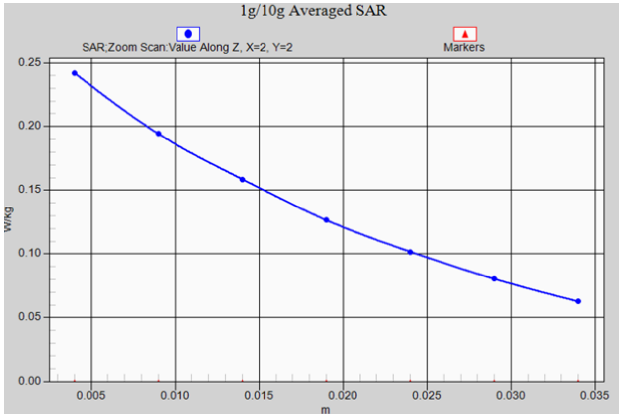
GSM850 RIGHT/CHEEK-High_ axis scan
