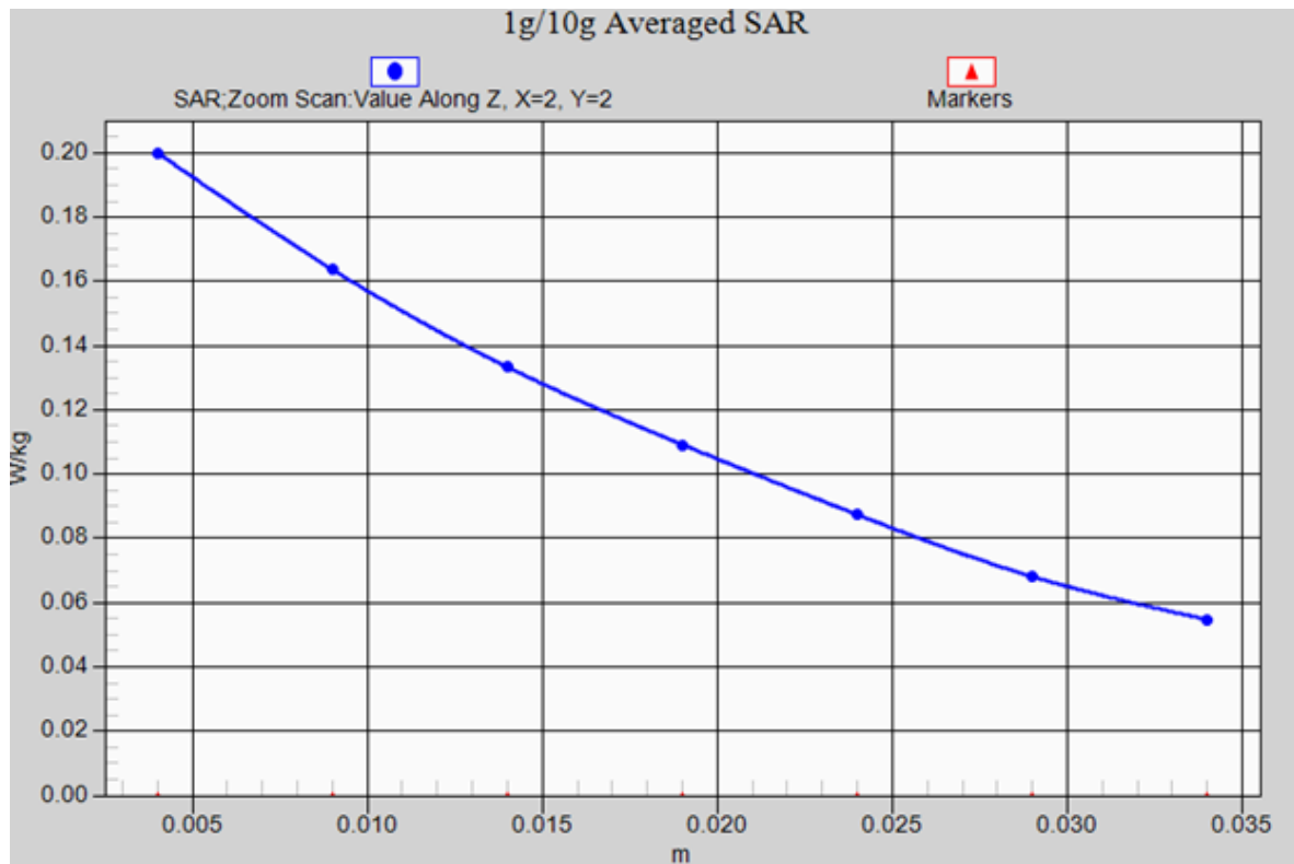
WCDMA Band V- LEFT/CHEEK-Mid- axis scan
