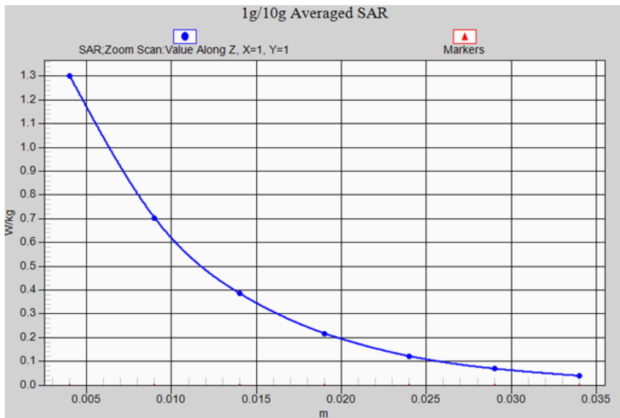
GPRS 1900/Back side-High_ axis scan
