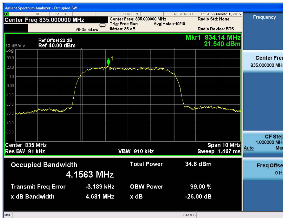
Fig.8 WCDMA Band V-CH4175 Occupied Bandwidth
