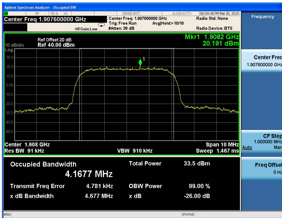
Fig.18 WCDMA Band II-CH9538 Occupied Bandwidth
