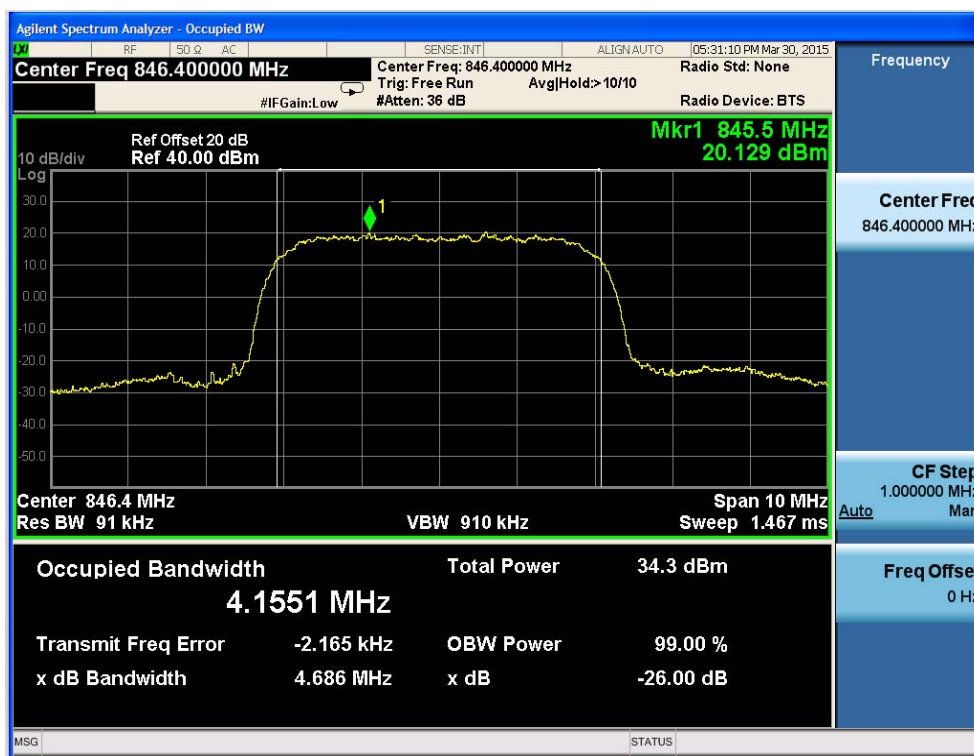
Fig.12 WCDMA Band V-CH4232 Occupied Bandwidth (HSDPA Subtest 1)
