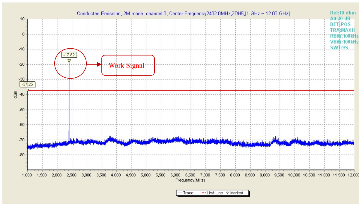
Fig.47 Conducted Emission in 2M mode ,channel 0, (1 GHz ~ 12 GHz)
