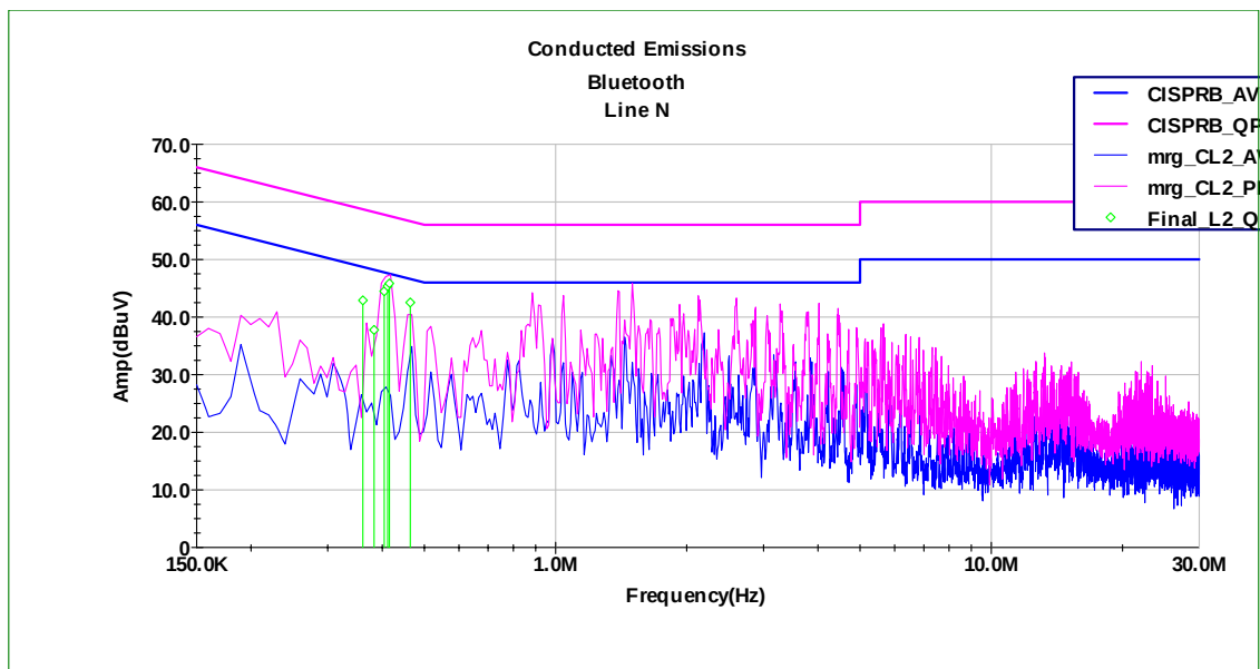
Line N
