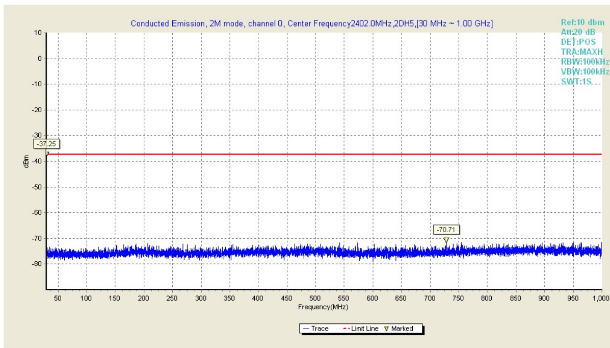
Fig.46 Conducted Emission in 2M mode ,channel 0, (30 MHz ~ 1 GHz)
