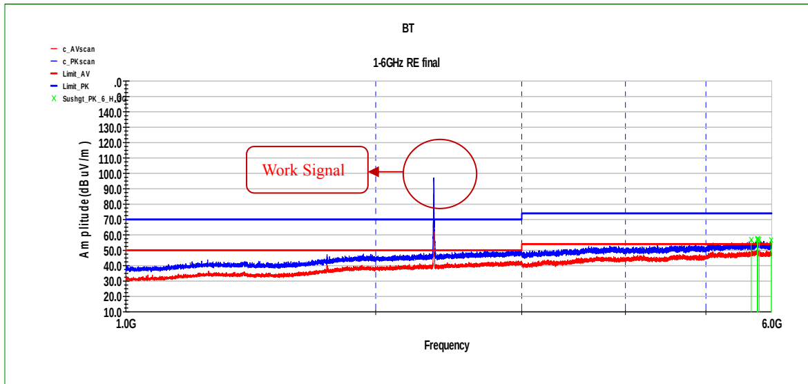
Fig.66 Radiated Emission of channel 0 in 1GHz-6GHz
