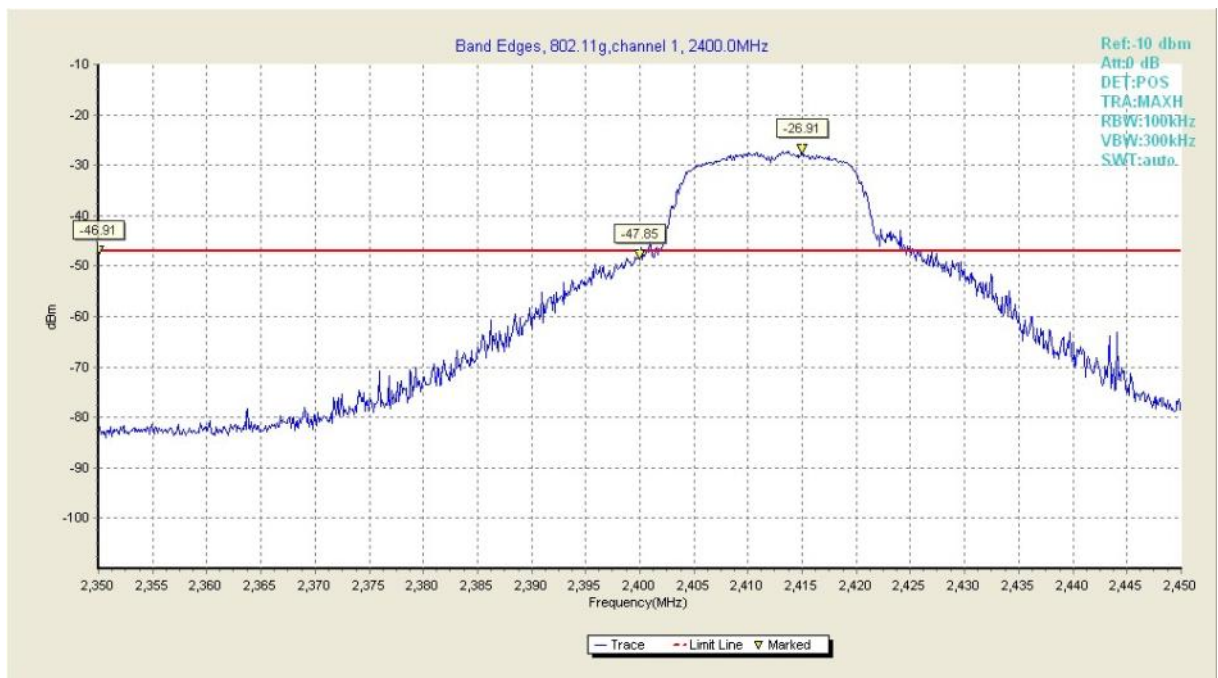
Fig27. Frequency Band Edges of 802.11g in channel 1, 2400MHz
