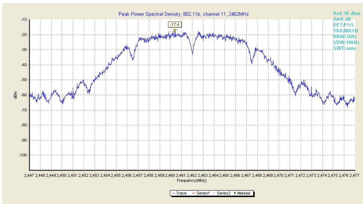
Fig.3 Peak power spectral density of 802.11b in channel 11,2462MHz
