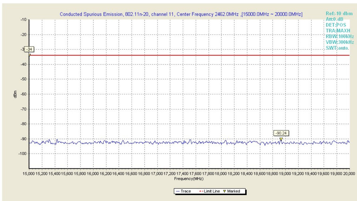
Fig94. Conducted Transmission Spurious Emission of 802.11n-20 in channel 11, 15GHz ~ 20GHz
