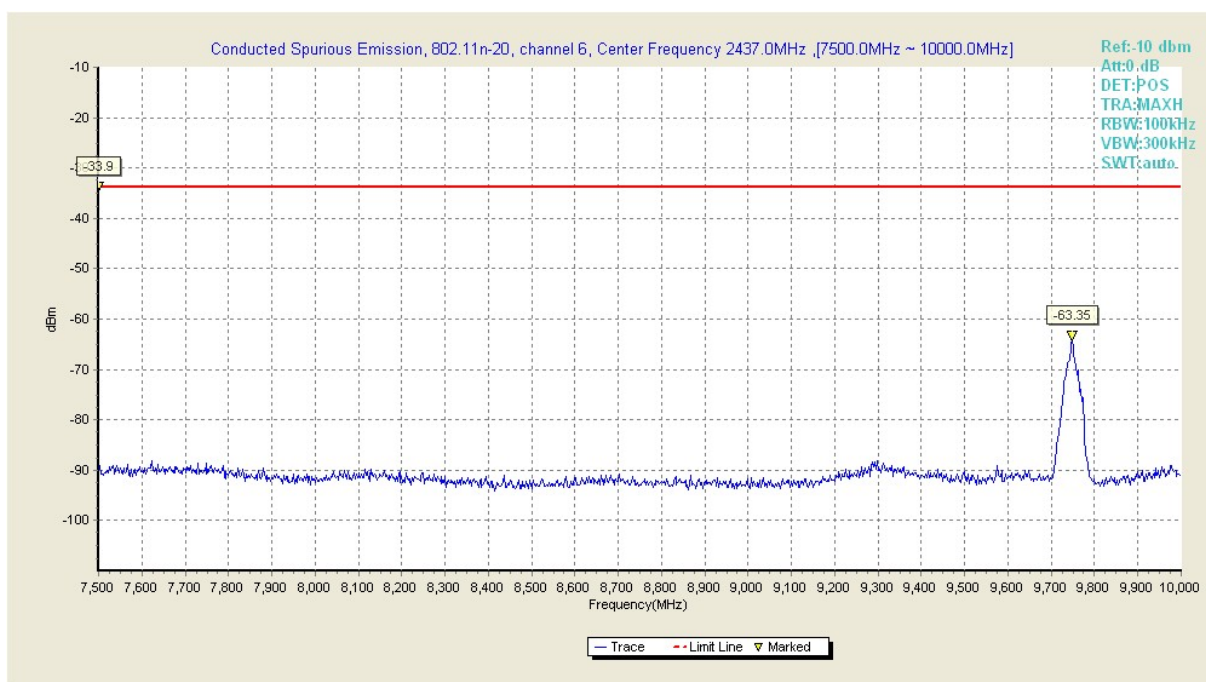
Fig85. Conducted Transmission Spurious Emission of 802.11n-20 in channel 6, 7.5GHz ~ 10GHz
