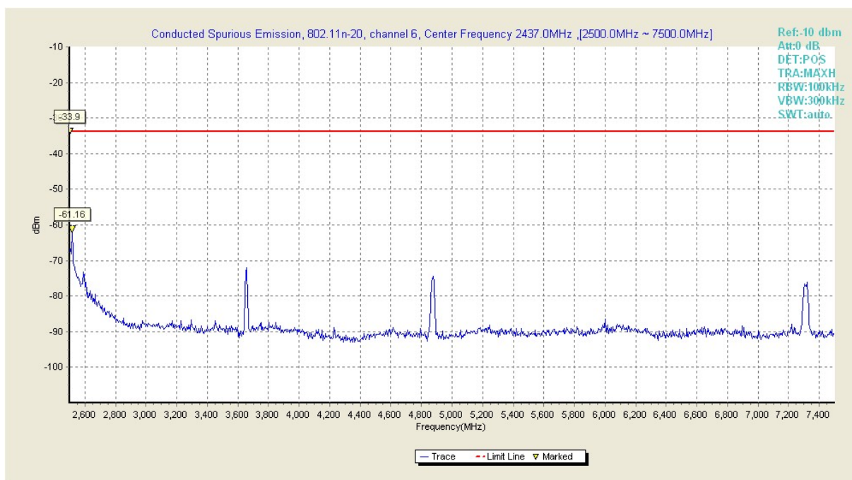
Fig84. Conducted Transmission Spurious Emission of 802.11n-20 in channel 6, 2.5GHz ~ 7.5GHz
