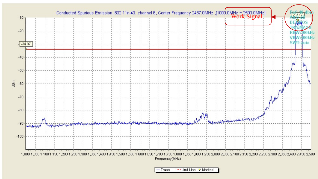
Fig104. Conducted Transmission Spurious Emission of 802.11n-40 in channel 6, 1GHz ~ 2.5GHz
