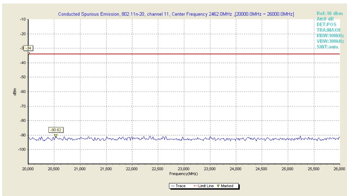
Fig95. Conducted Transmission Spurious Emission of 802.11n-20 in channel 11, 20GHz ~ 26GHz
