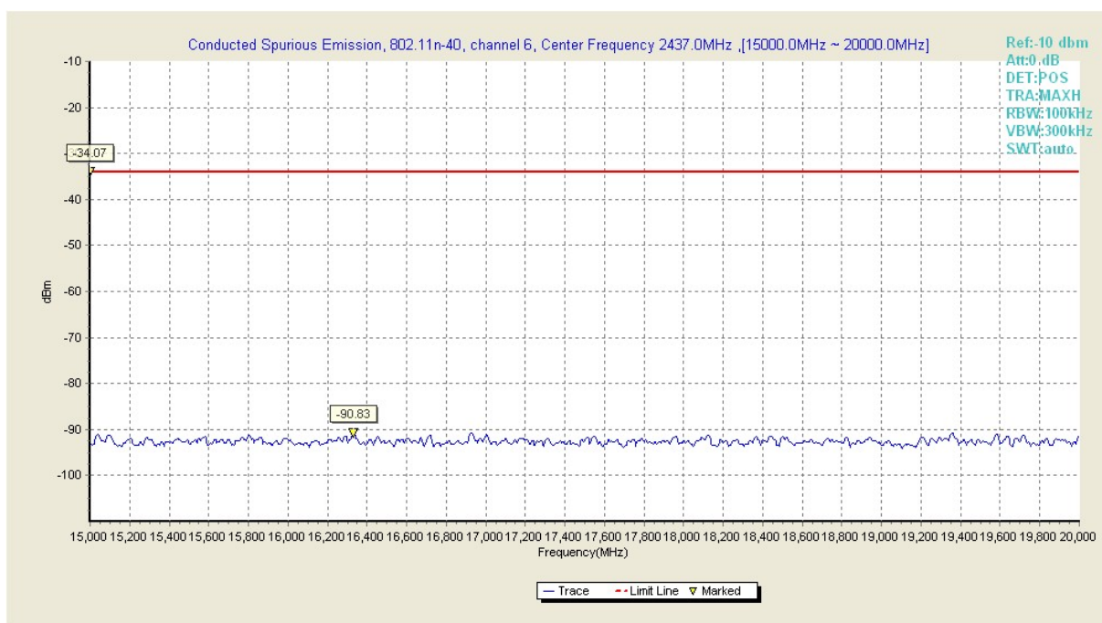
Fig108. Conducted Transmission Spurious Emission of 802.11n-40 in channel 6, 15GHz ~ 20GHz
