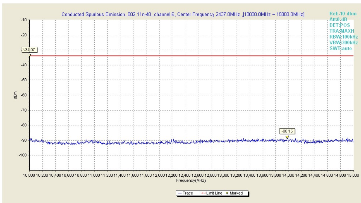
Fig107. Conducted Transmission Spurious Emission of 802.11n-40 in channel 6, 10GHz ~ 15GHz
