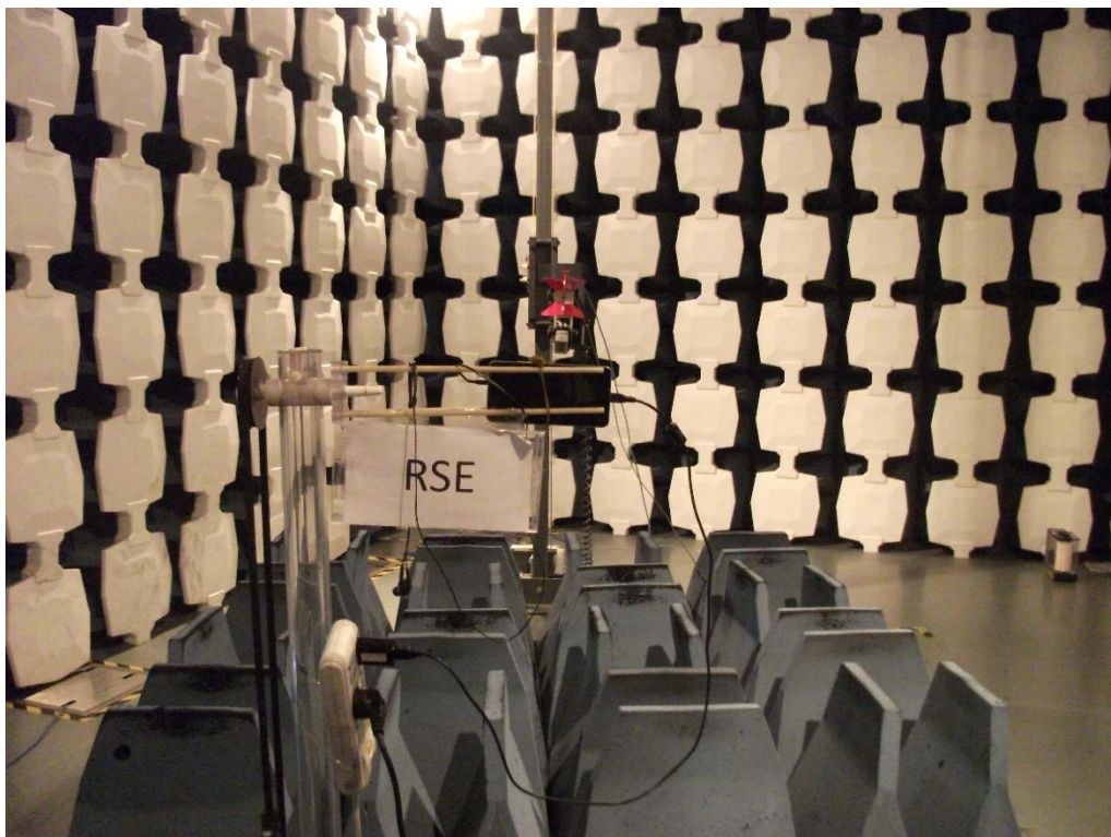
RSE Above 3GHz
