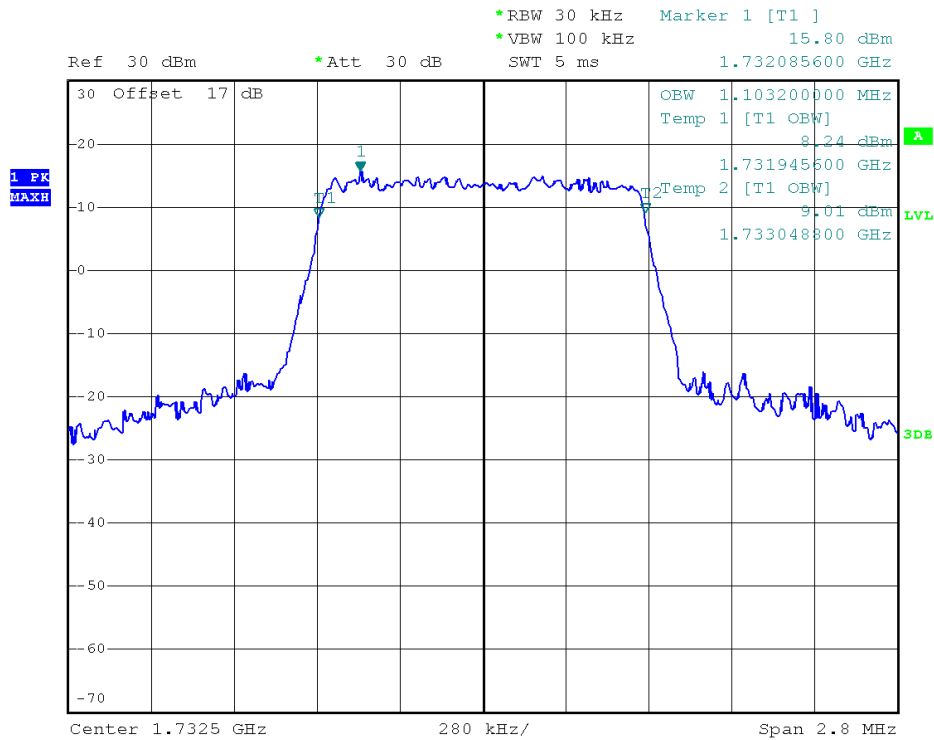
(Plot G3: 99% Occupied Bandwidth LTE Band 4/1.4MHz/16QAM)
