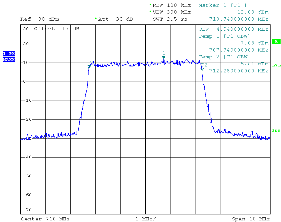
(Plot Q3: 99% Occupied Bandwidth LTE Band 17/5MHz/16QAM)
