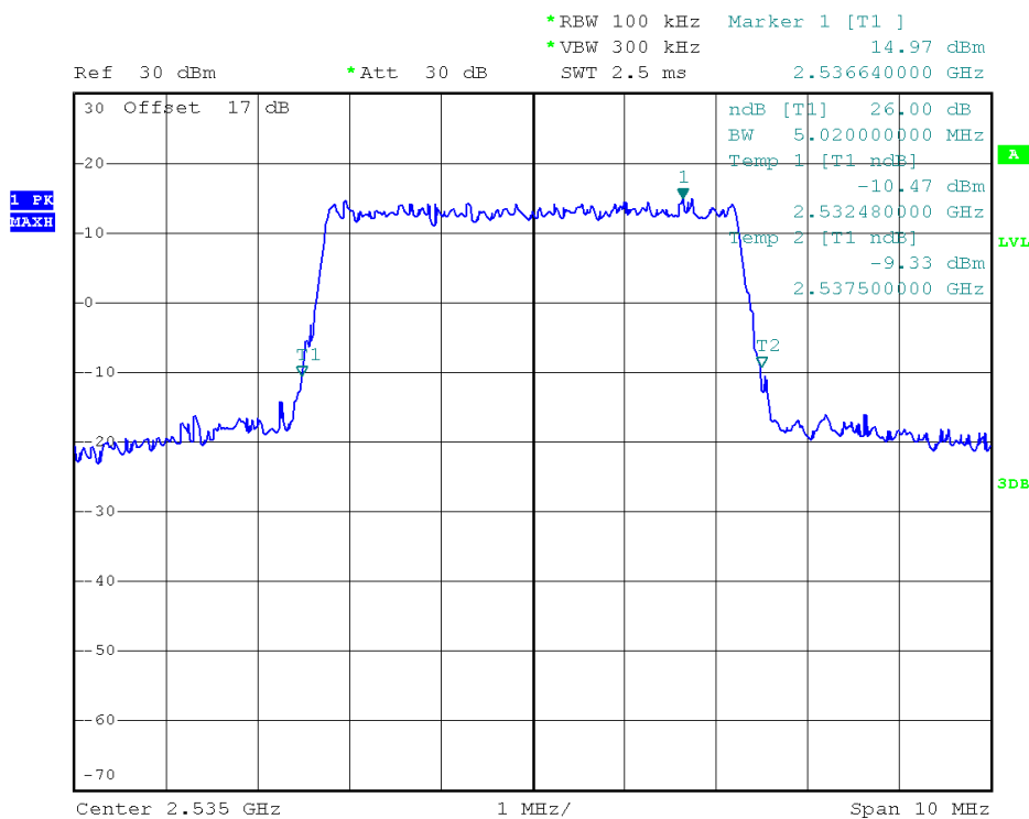
(Plot M4: 26dB Bandwidth LTE Band 7/5MHz/16QAM)
