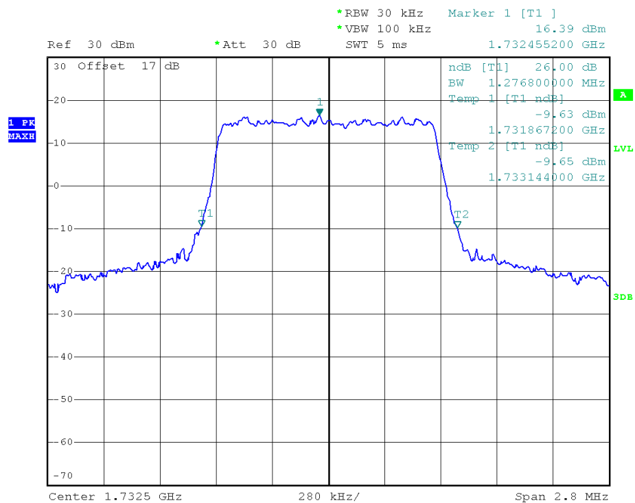
(Plot G2: 26dB Bandwidth LTE Band 4/1.4MHz/QPSK)
