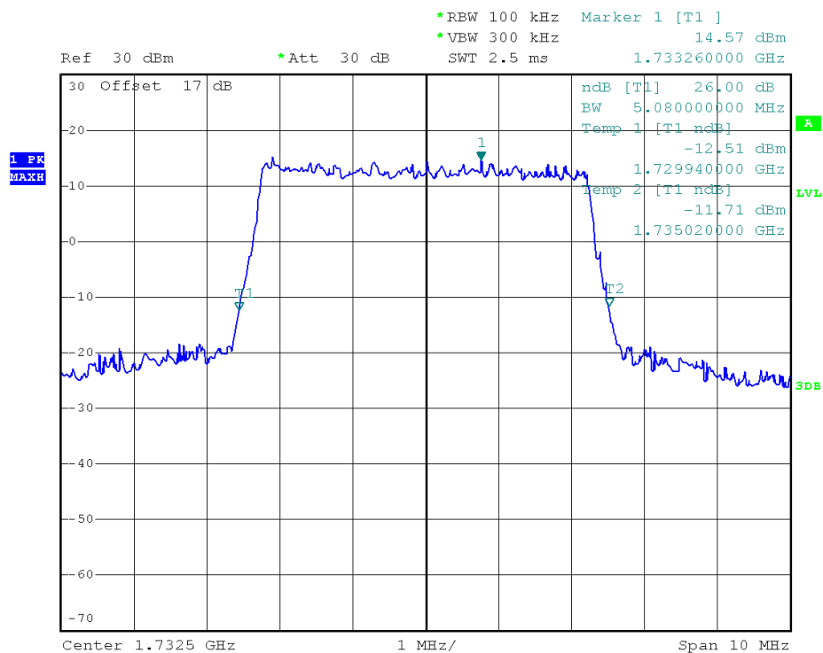
(Plot I4: 26dB Bandwidth LTE Band 4/5MHz/16QAM)
