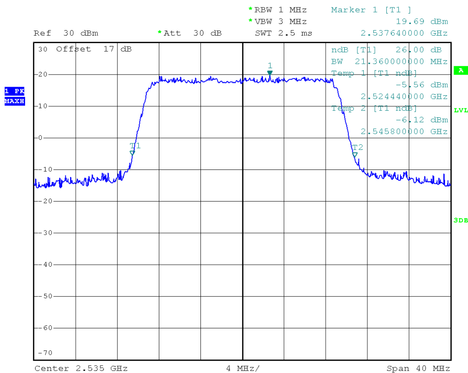
(Plot P2: 26dB Bandwidth LTE Band 7/20MHz/QPSK)
