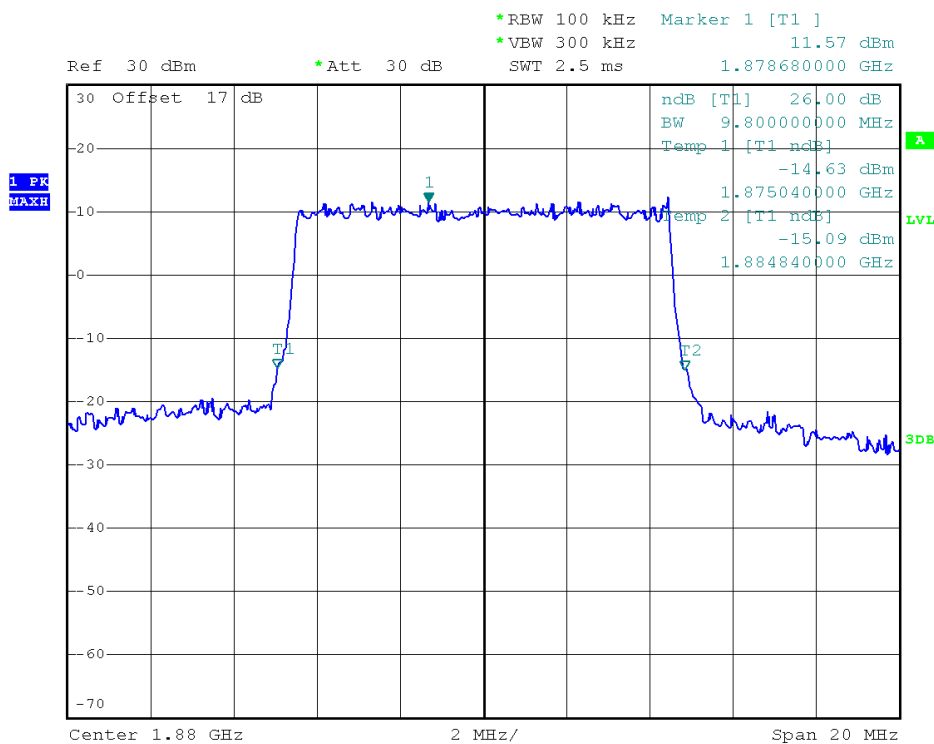
(Plot D4: 26dB Bandwidth LTE Band 2/10MHz/16QAM)
