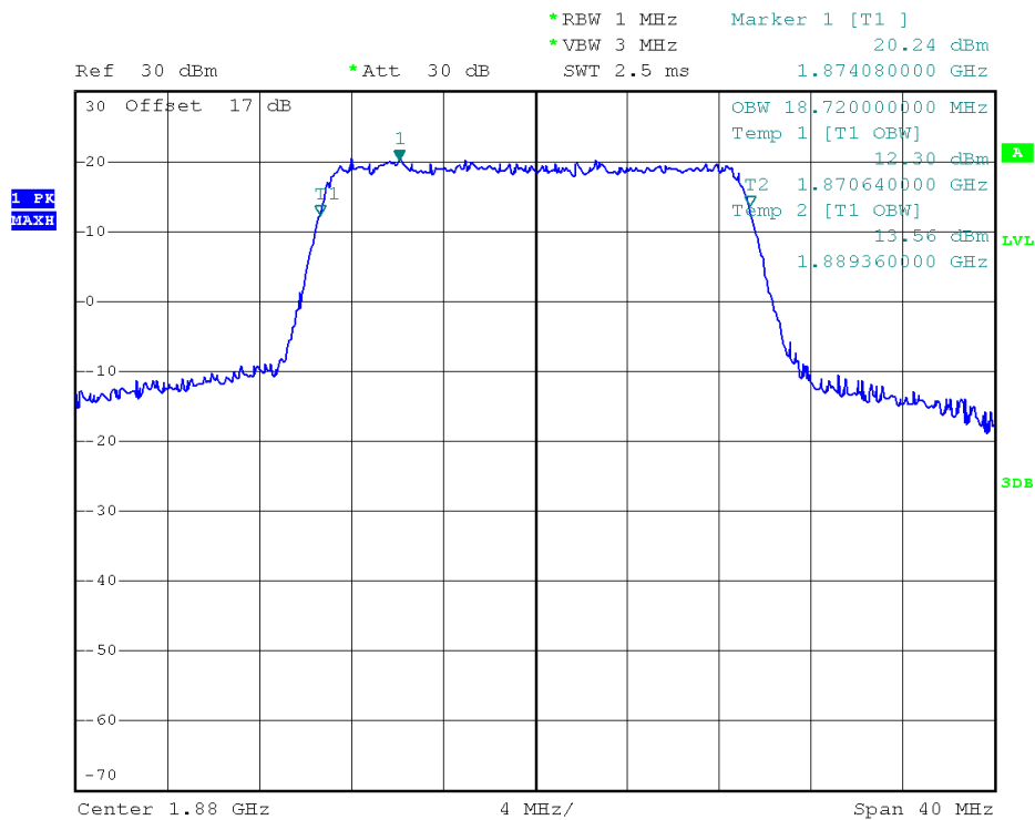
(Plot F1: 99% Occupied Bandwidth LTE Band 2/20MHz/QPSK)
