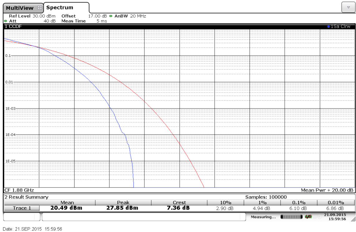
(Plot A4: Band 2/20MHz/16QAM in Ch.18900 100RB Size)
