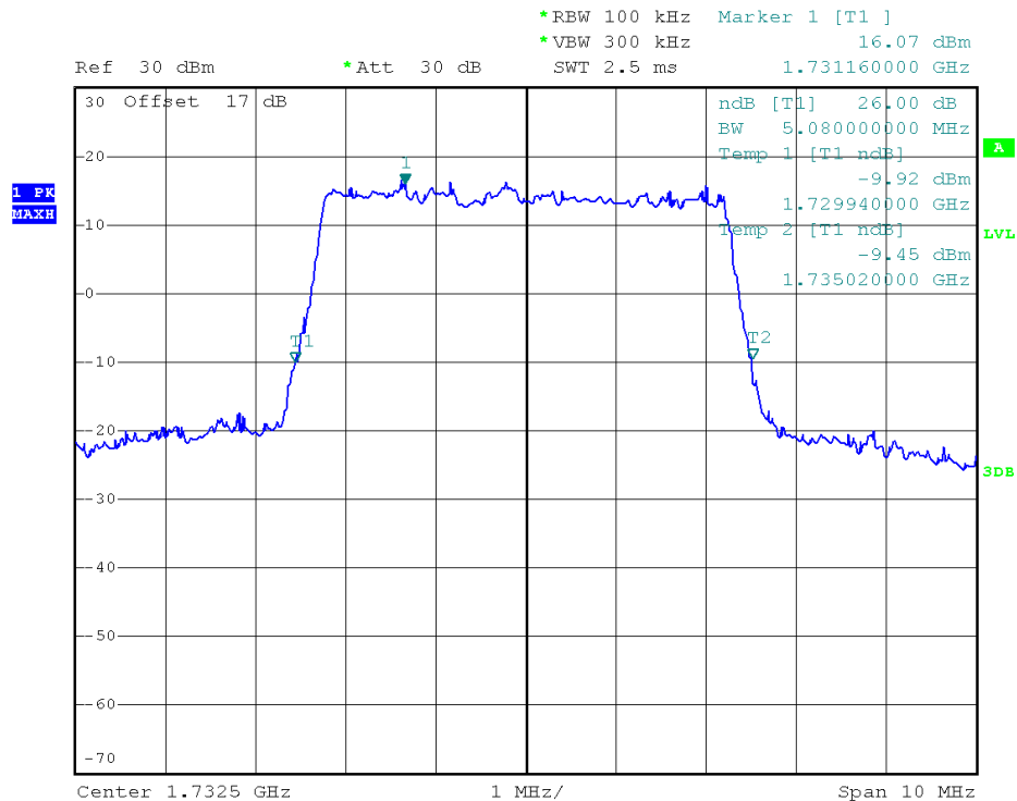
(Plot I2: 26dB Bandwidth LTE Band 4/5MHz/QPSK)
