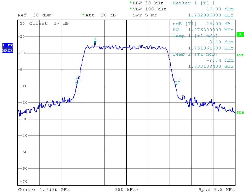
(Plot G4: 26dB Bandwidth LTE Band 4/1.4MHz/16QAM)
