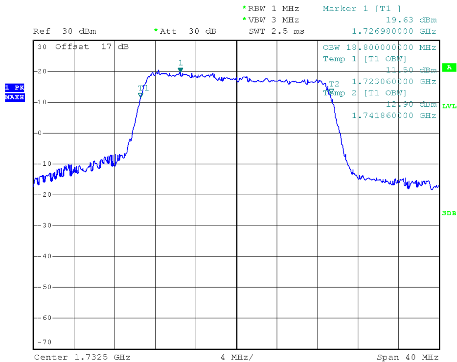
(Plot L3: 99% Occupied Bandwidth LTE Band 4/20MHz/16QAM)
