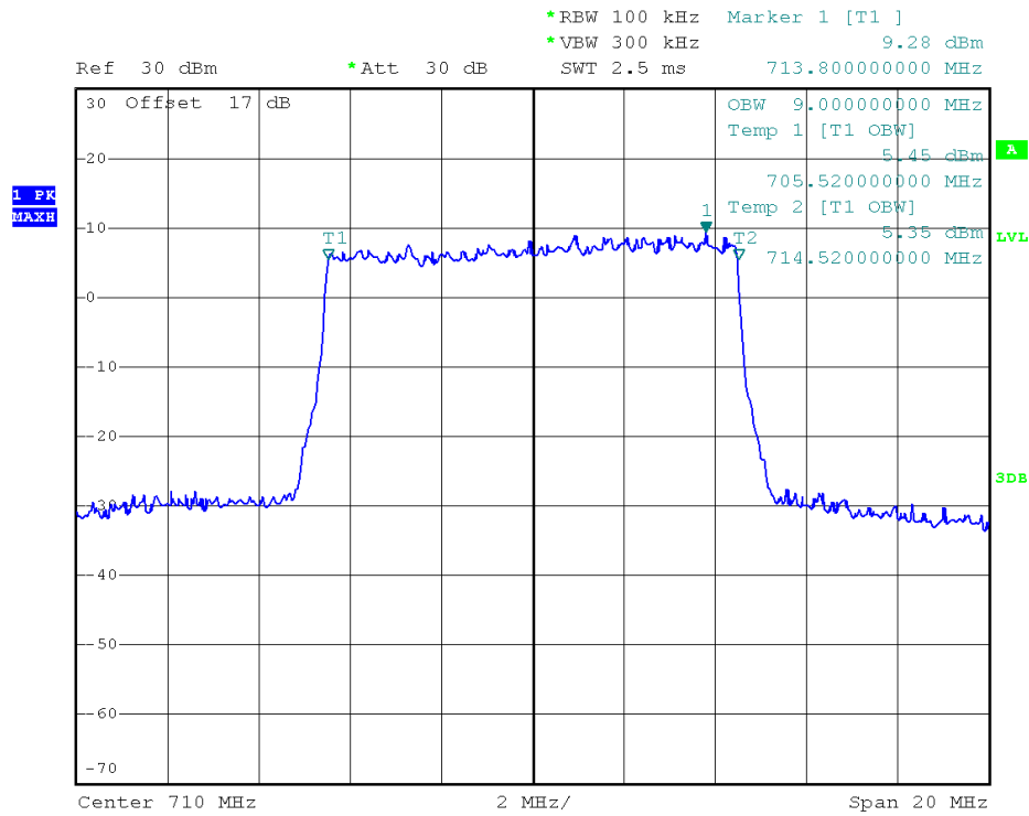
(Plot R3: 99% Occupied Bandwidth LTE Band17/10MHz/16QAM)
