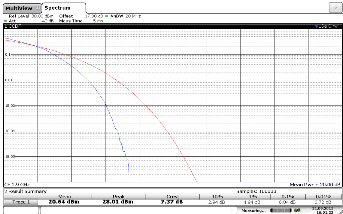
(Plot A6: Band 2/20MHz/16QAM in Ch.19100 100RB Size)
