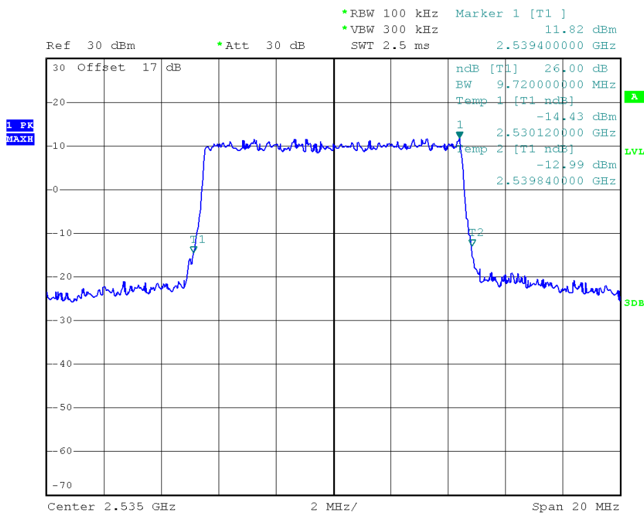
(Plot N4: 26dB Bandwidth LTE Band 7/10MHz/16QAM)
