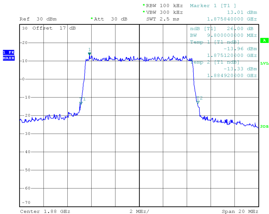
(Plot D2: 26dB Bandwidth LTE Band 2/10MHz/QPSK)
