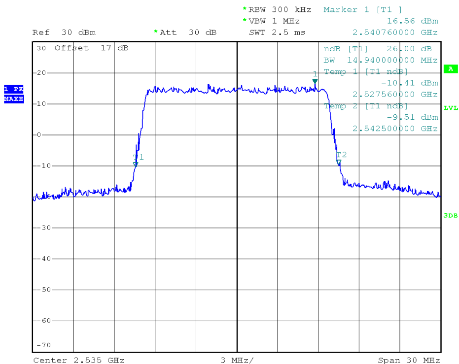
(Plot O2: 26dB Bandwidth LTE Band 7/15MHz/QPSK)
