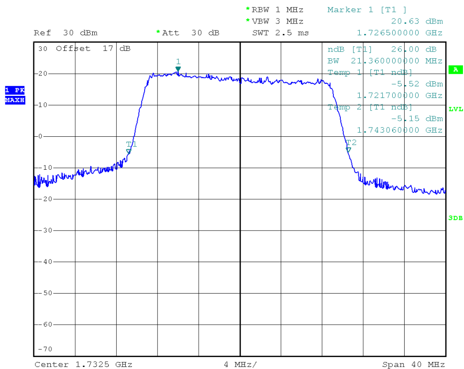
(Plot L2: 26dB Bandwidth LTE Band 4/20MHz/QPSK)
