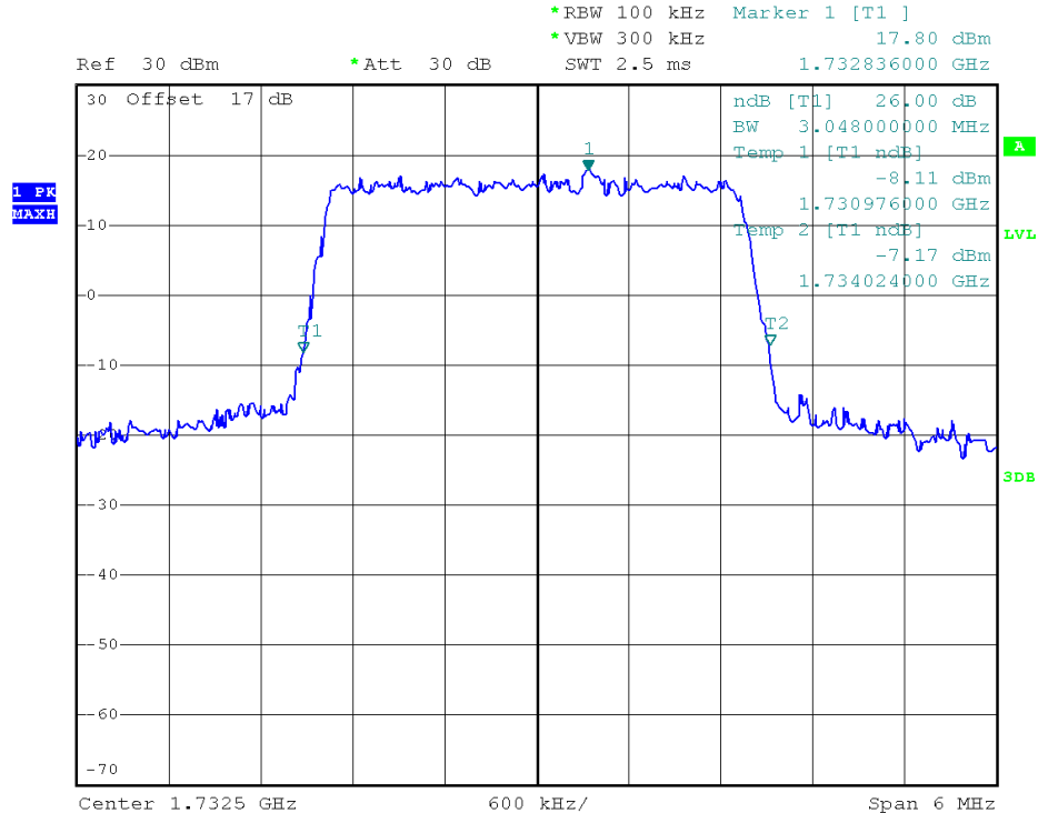
(Plot H2: 26dB Bandwidth LTE Band 4/3MHz/QPSK)
