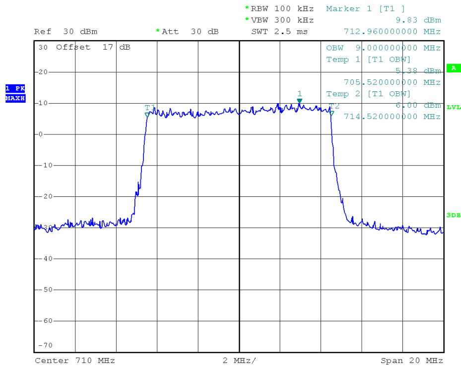
(Plot R1: 99% Occupied Bandwidth LTE Band 17/10MHz/QPSK)
