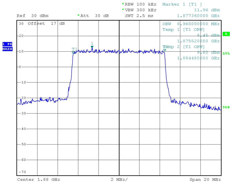
(Plot D3: 99% Occupied Bandwidth LTE Band 2/10MHz/16QAM)
