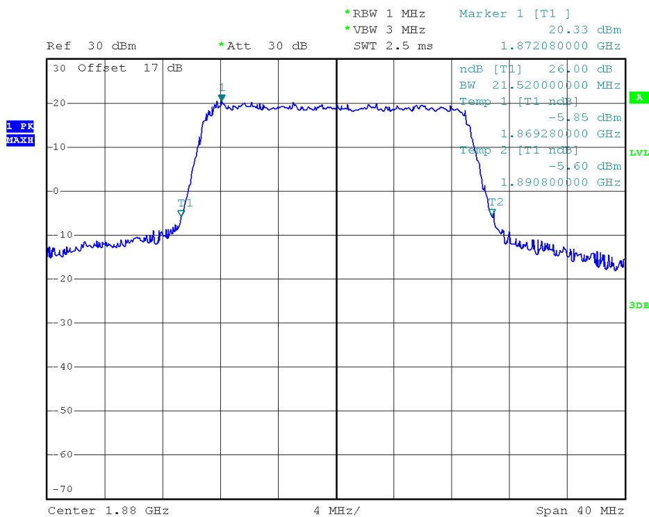
(Plot F2: 26dB Bandwidth LTE Band 2/20MHz/QPSK)
