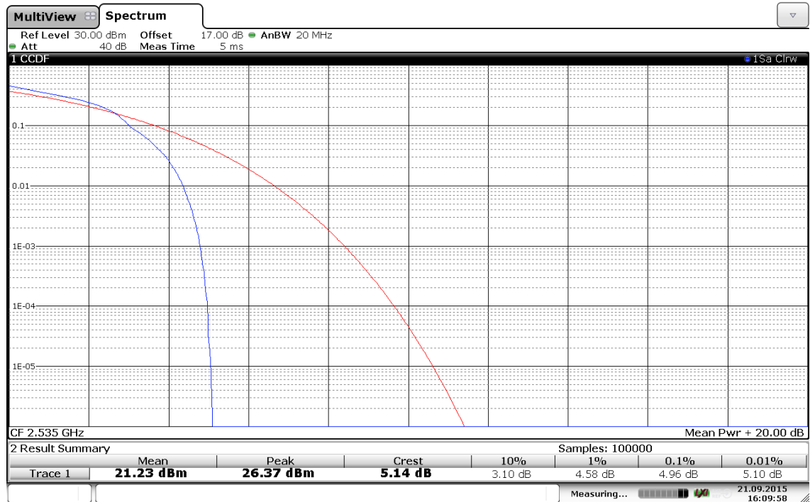
(Plot C3: Band 7/20MHz/16QAM in Ch.21100 1RB Size)
