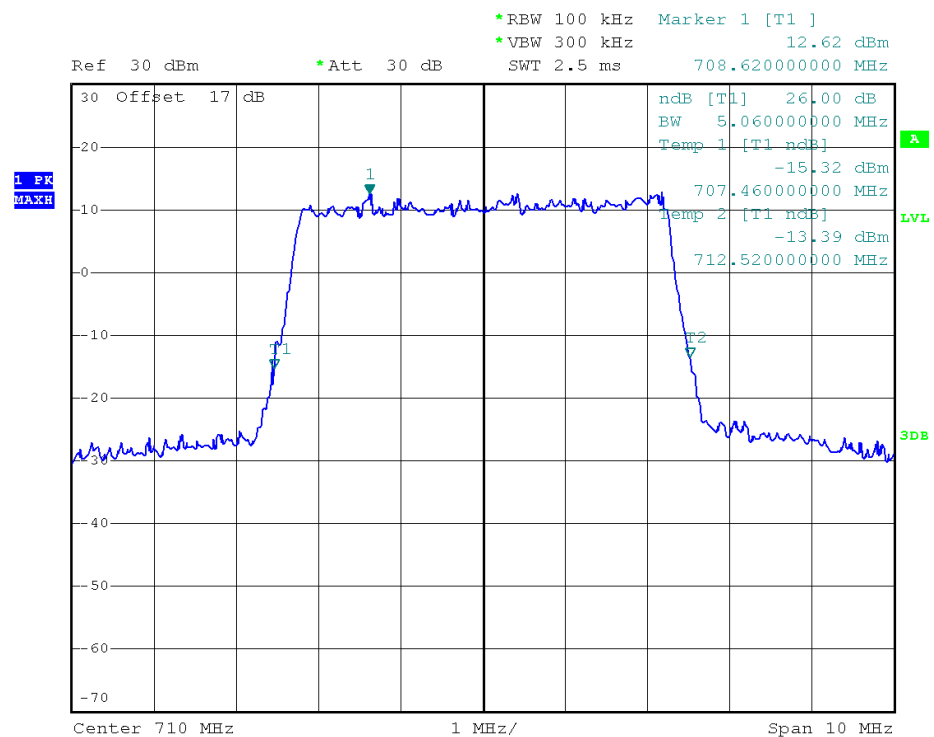
(Plot Q2: 26dB Bandwidth LTE Band 17/5MHz/QPSK)
