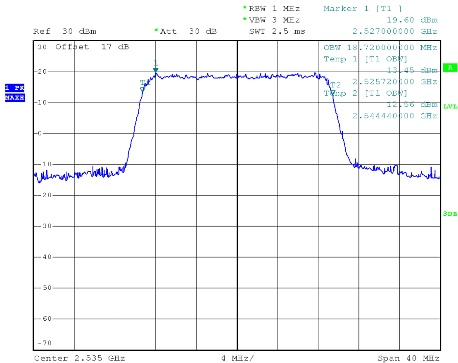
(Plot P1: 99% Occupied Bandwidth LTE Band 7/20MHz/QPSK)
