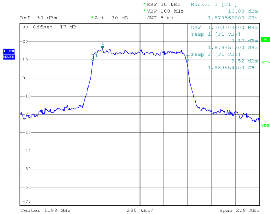
(Plot A3: 99% Occupied Bandwidth LTE Band 2 1.4MHz/16QAM)
