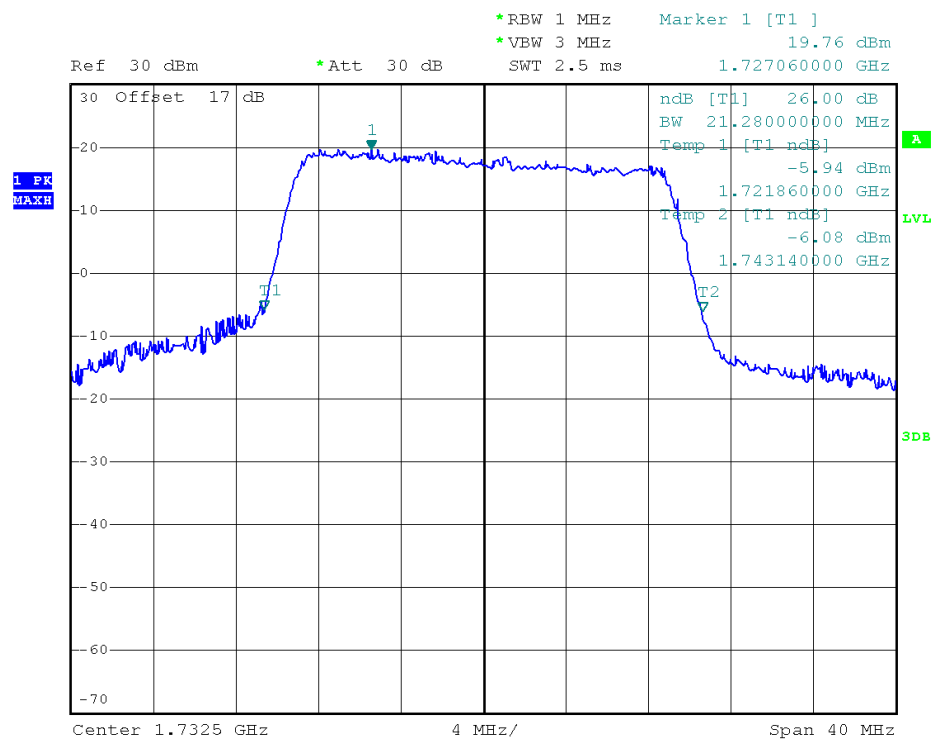
(Plot L4: 26dB Bandwidth LTE Band 4/20MHz/16QAM)
