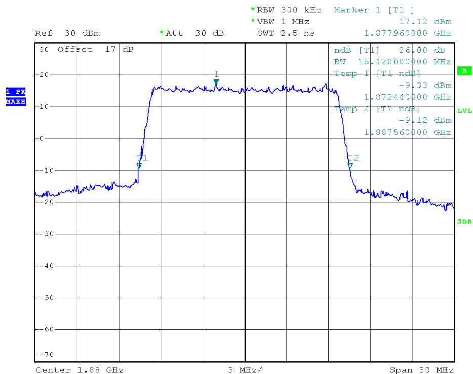
(Plot E2: 26dB Bandwidth LTE Band 2/15MHz/QPSK)
