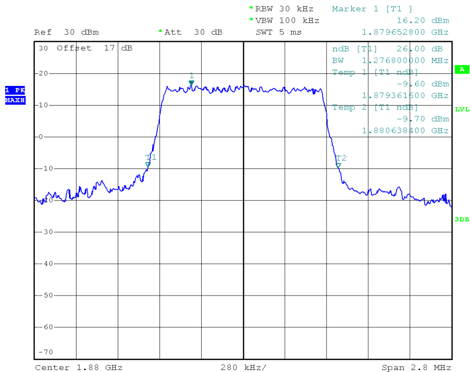
(Plot A2: 26dB Bandwidth LTE Band 2 1.4MHz/QPSK)
