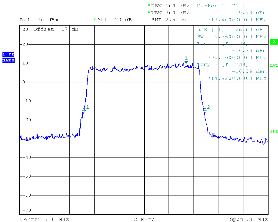
(Plot R2: 26dB Bandwidth LTE Band17/10MHz/QPSK)
