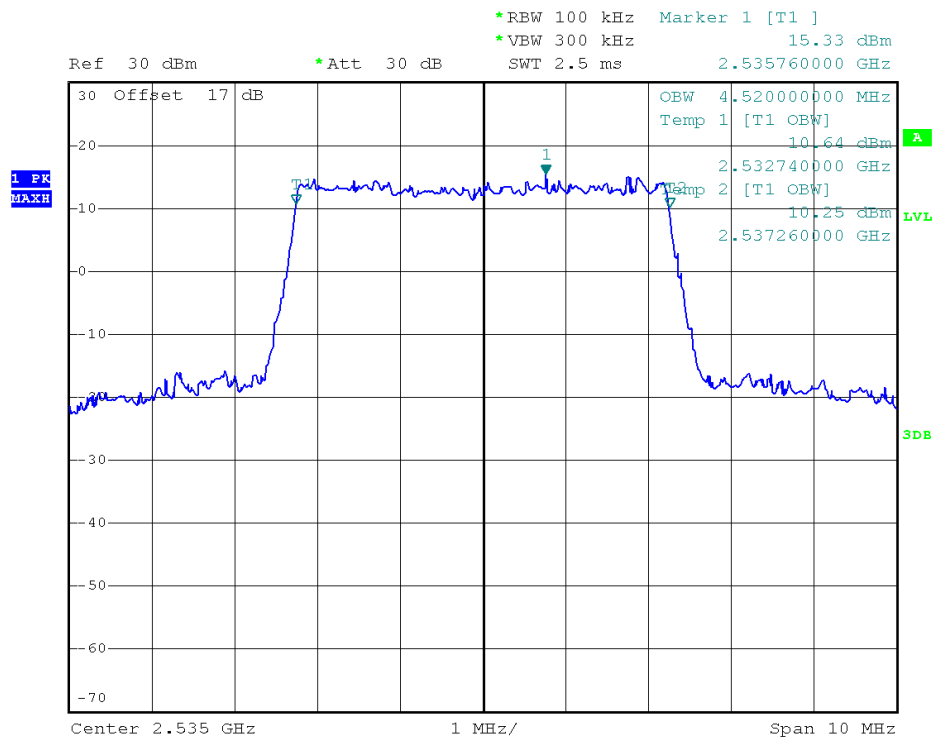
(Plot M3: 99% Occupied Bandwidth LTE Band 7/5MHz/16QAM)
