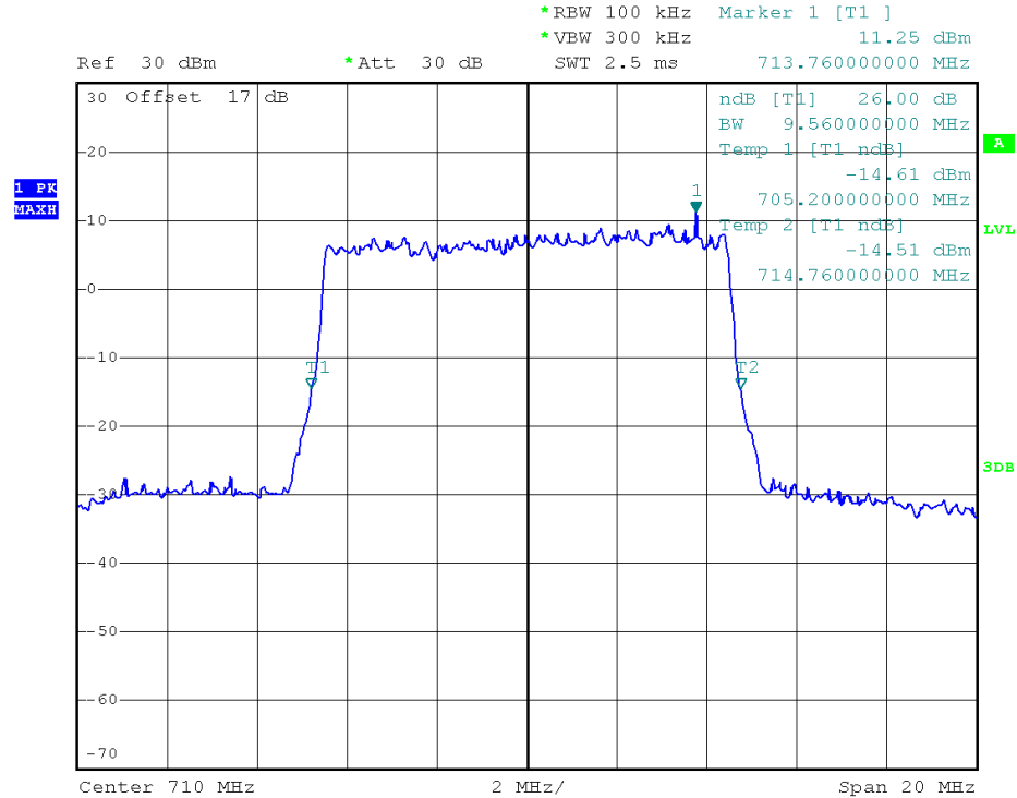
(Plot R4: 26dB Bandwidth LTE Band17/10MHz/16QAM)
