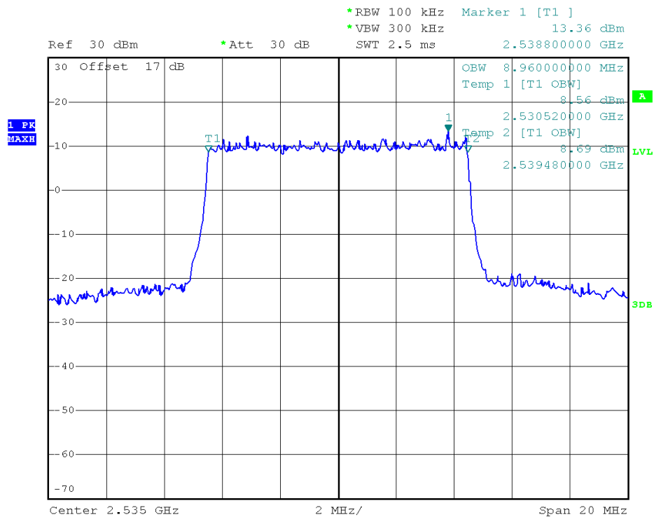
(Plot N3: 99% Occupied Bandwidth LTE Band 7/10MHz/16QAM)
