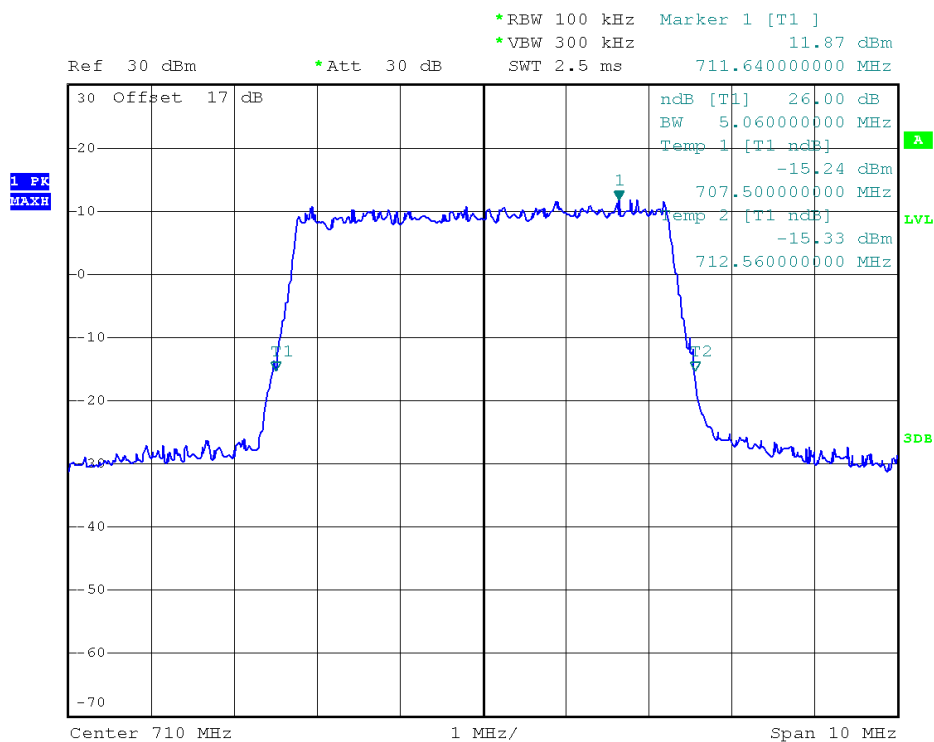
(Plot Q4: 26dB Bandwidth LTE Band 17/5MHz/16QAM)
