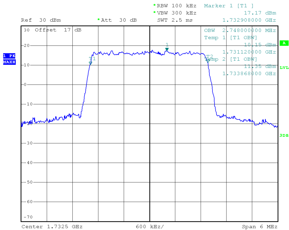
(Plot H1: 99% Occupied Bandwidth LTE Band 4/3MHz/QPSK)
