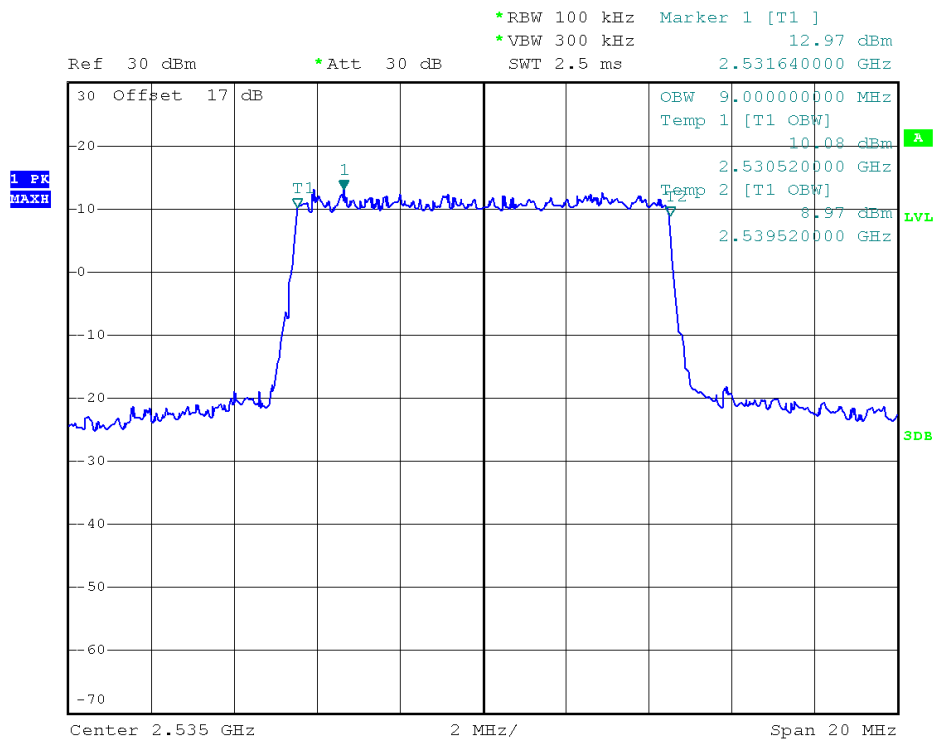
(Plot N1: 99% Occupied Bandwidth LTE Band 7/10MHz/QPSK)
