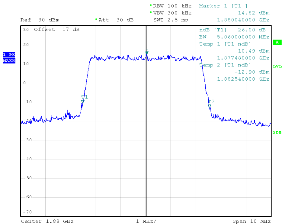
(Plot C4: 26dB Bandwidth LTE Band 2/5MHz/16QAM)
