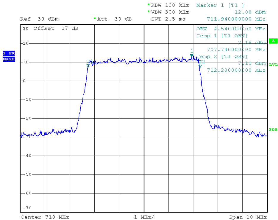
(Plot Q1: 99% Occupied Bandwidth LTE Band 17/5MHz/QPSK)
