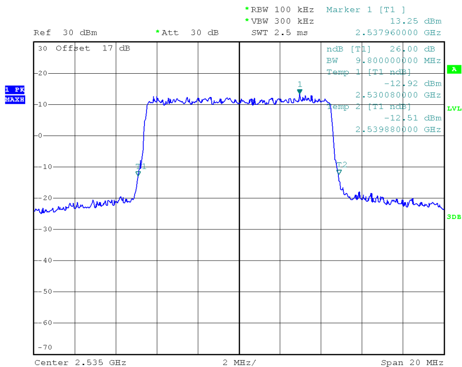
(Plot N2: 26dB Bandwidth LTE Band 7/10MHz/QPSK)
