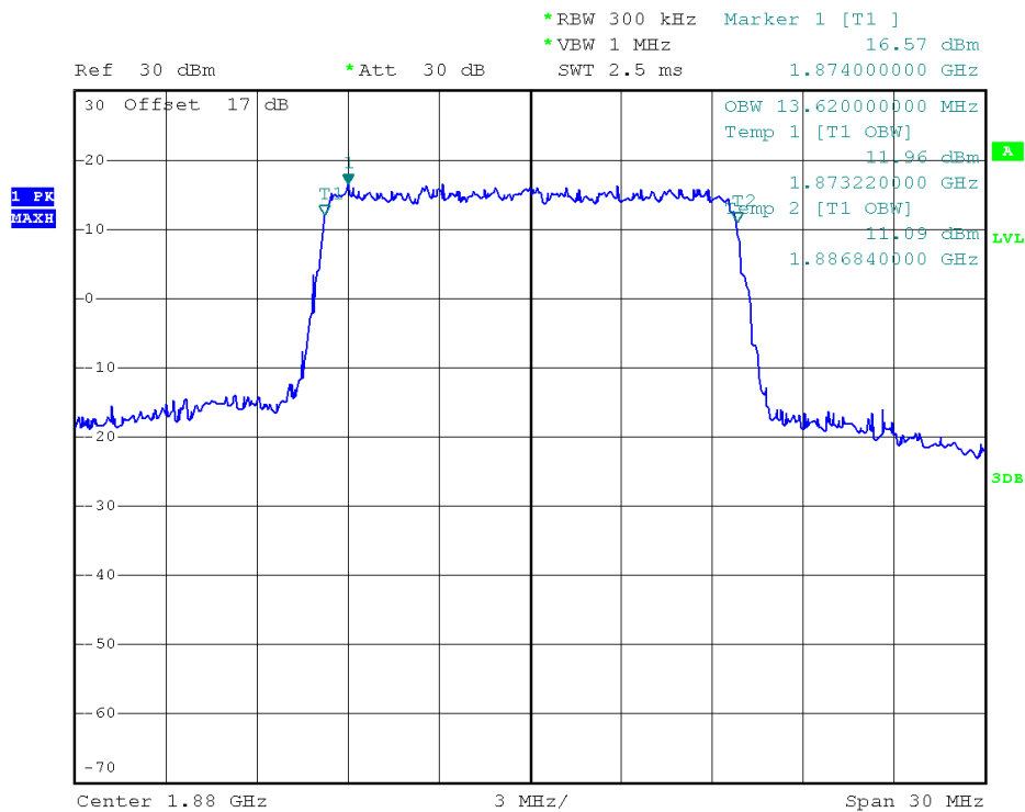
(Plot E1: 99% Occupied Bandwidth LTE Band 2/15MHz/QPSK)
