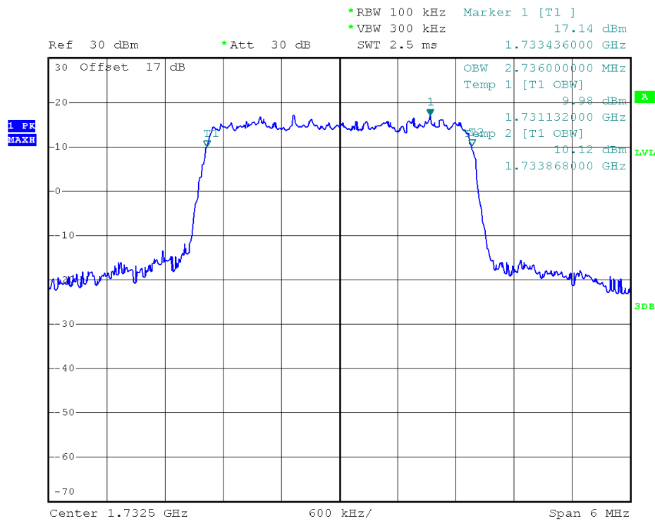
(Plot H3: 99% Occupied Bandwidth LTE Band 4/3MHz/16QAM)
