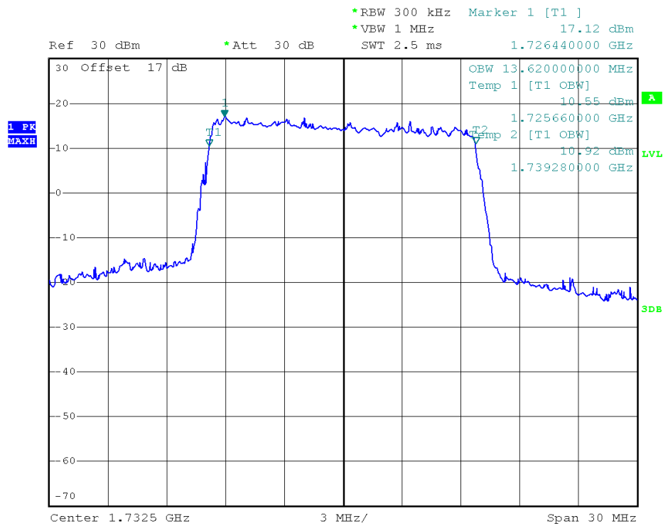
(Plot K1: 99% Occupied Bandwidth LTE Band 4/15MHz/QPSK)
