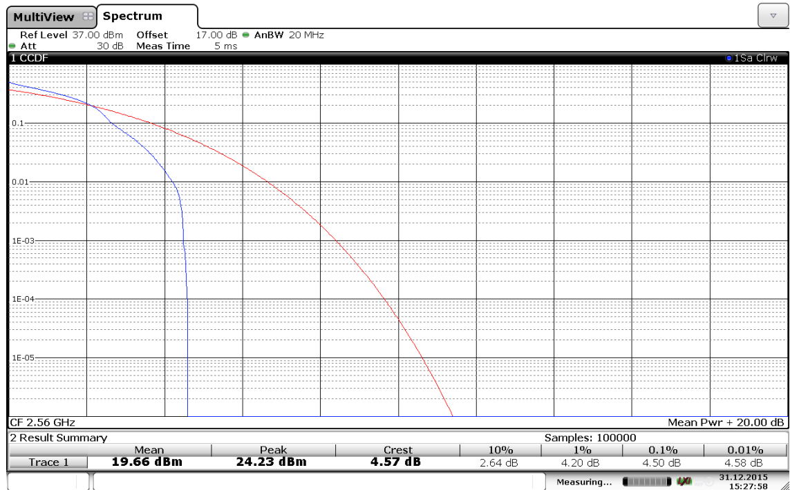
(Plot C5: Band 7/20MHz/16QAM in Ch.21350 1RB Size)
