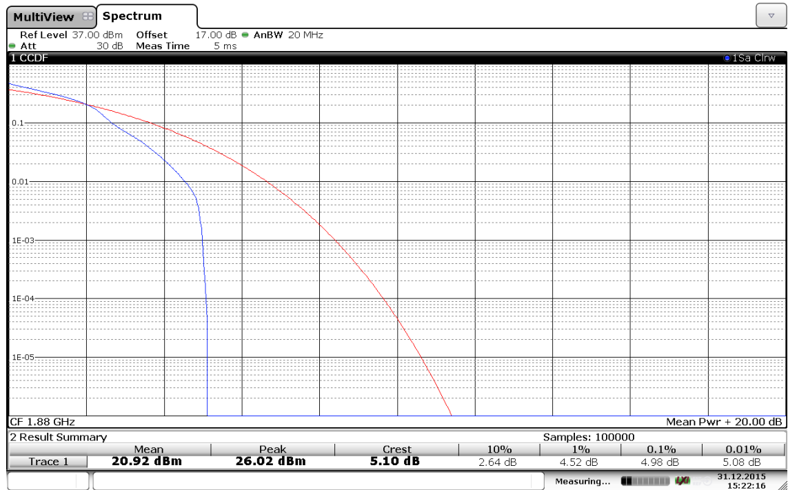
(Plot A3: Band 2/20MHz/16QAM in Ch.18900 1RB Size)
