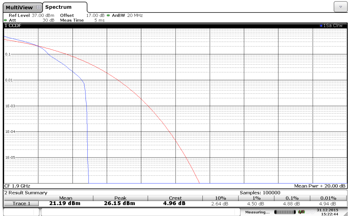
(Plot A5: Band 2/20MHz/16QAM in Ch.19100 1RB Size)
