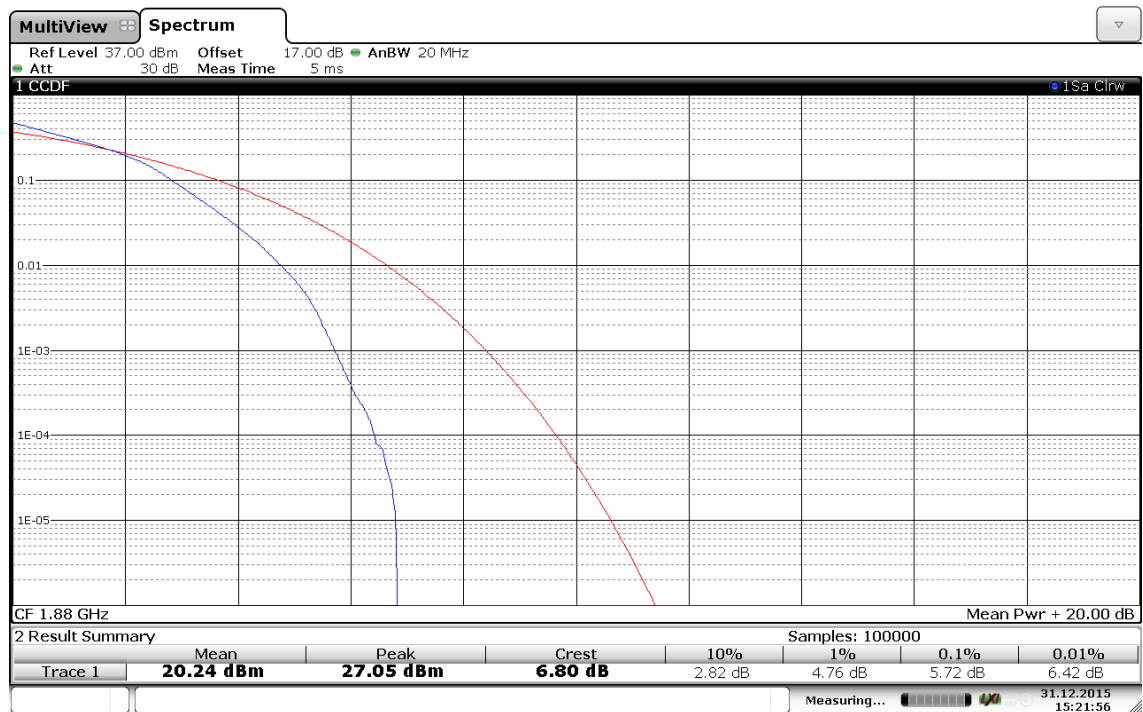
(Plot A4: Band 2/20MHz/16QAM in Ch.18900 100RB Size)
