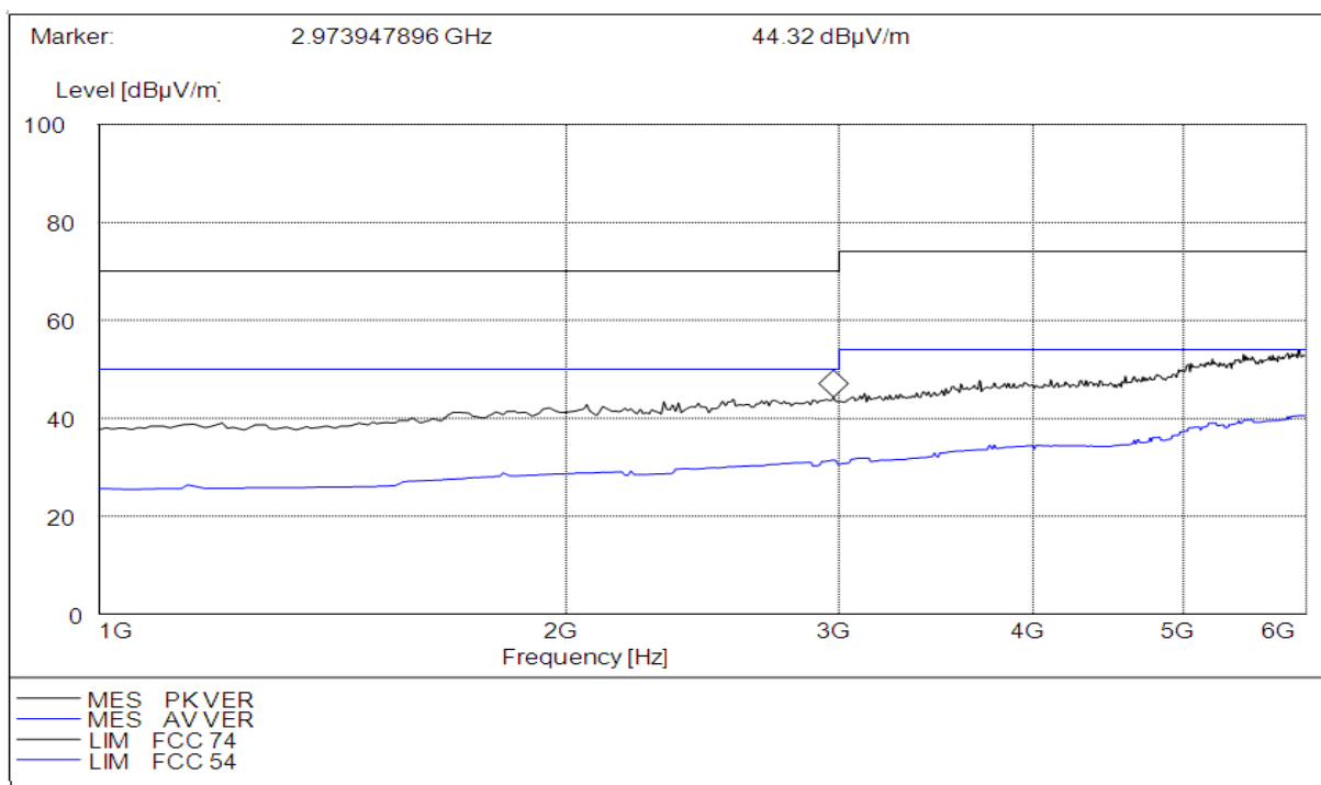
(Plot F: Test Antenna Vertical 1G – 6G)
