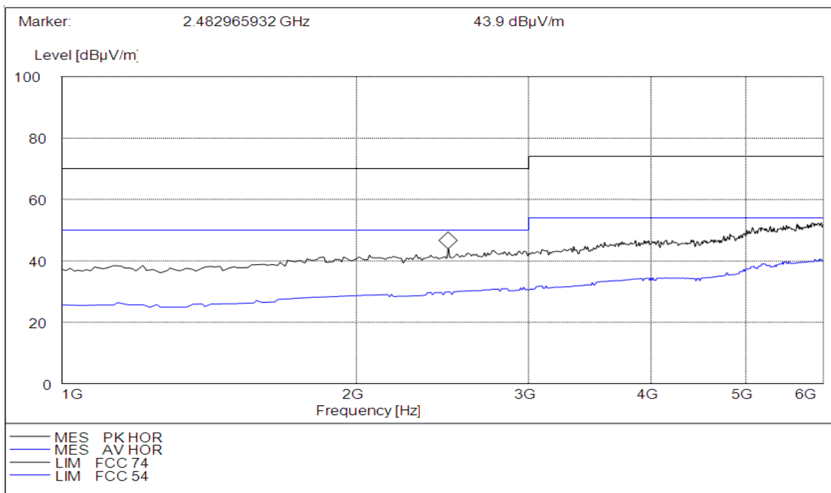
(Plot E: Test Antenna Horizontal 1G – 6G)
