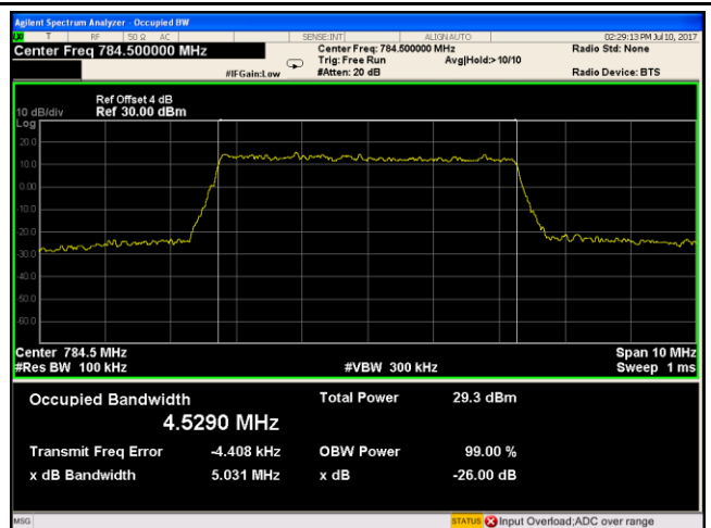
LTE band XIII - High CH 16QAM-5
