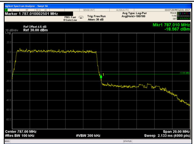
LTE band XIII - High Channel 16QAM-10
