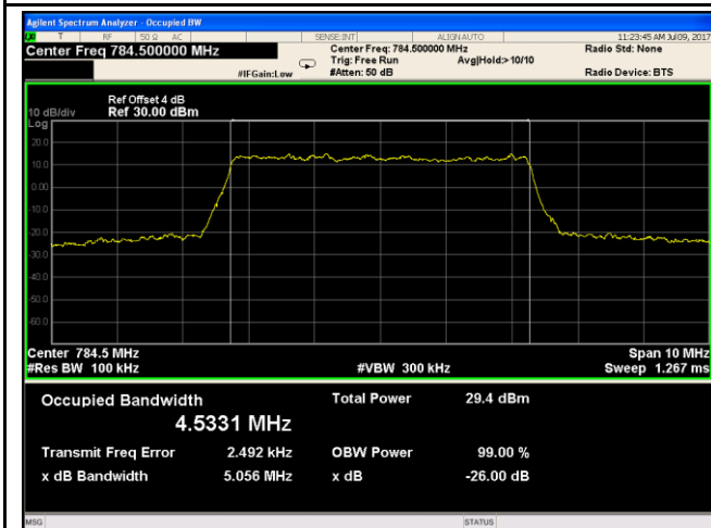
LTE band XIII - High CH QPSK-5
