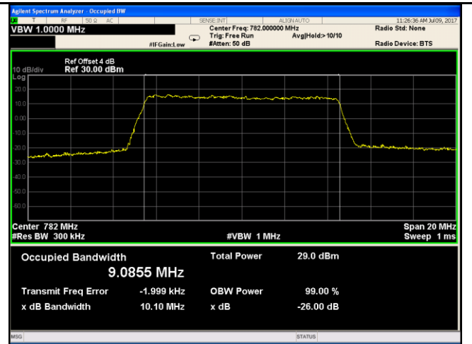
LTE band XIII - Low CH 16QAM-10
