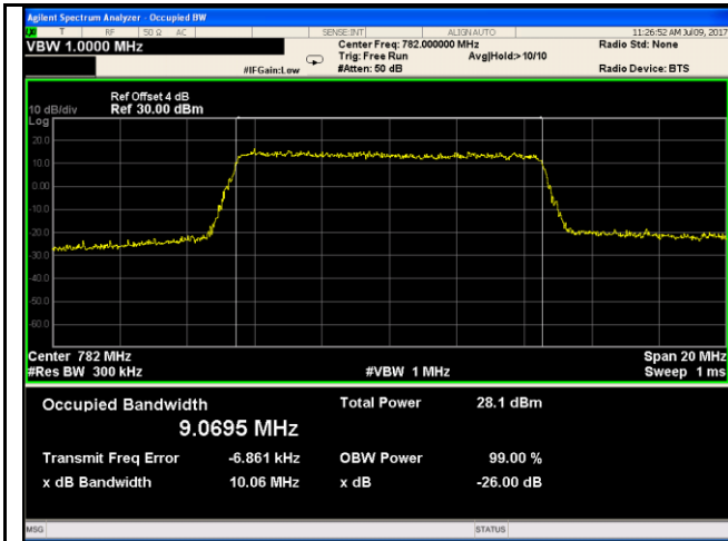
LTE band XIII - Low CH QPSK-10
