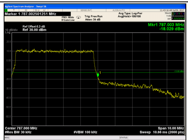
LTE band XIII - High Channel 16QAM-5
