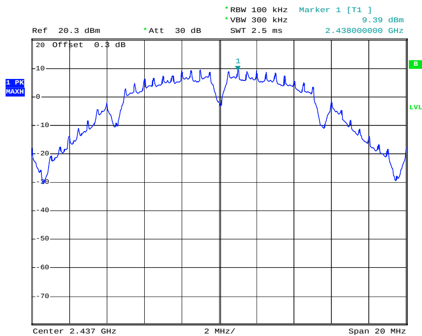
Mode 2 : PSD Plot on 802.11b Channel 06
