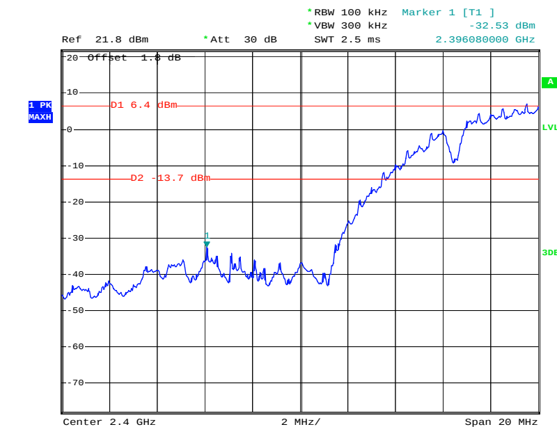
Low Band Edge Plot on 802.11b Channel 01
