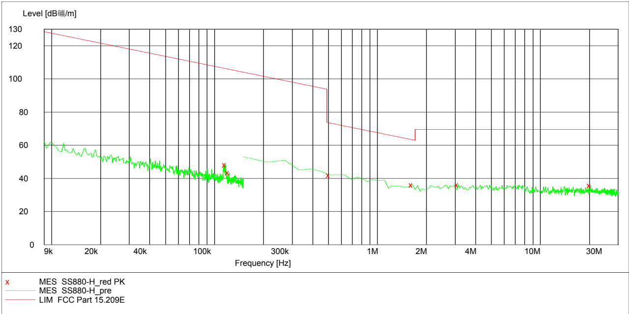
Radiated Emission Plot between 9 kHz ~ 30MHz (Horizontal)
