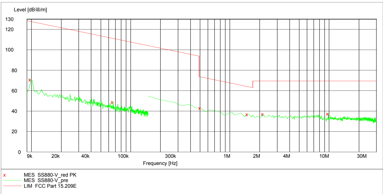
Radiated Emission Plot between 9 kHz ~ 30MHz (Vertical)
