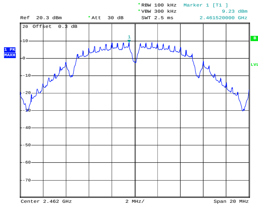
Mode 3 : PSD Plot on 802.11b Channel 11
