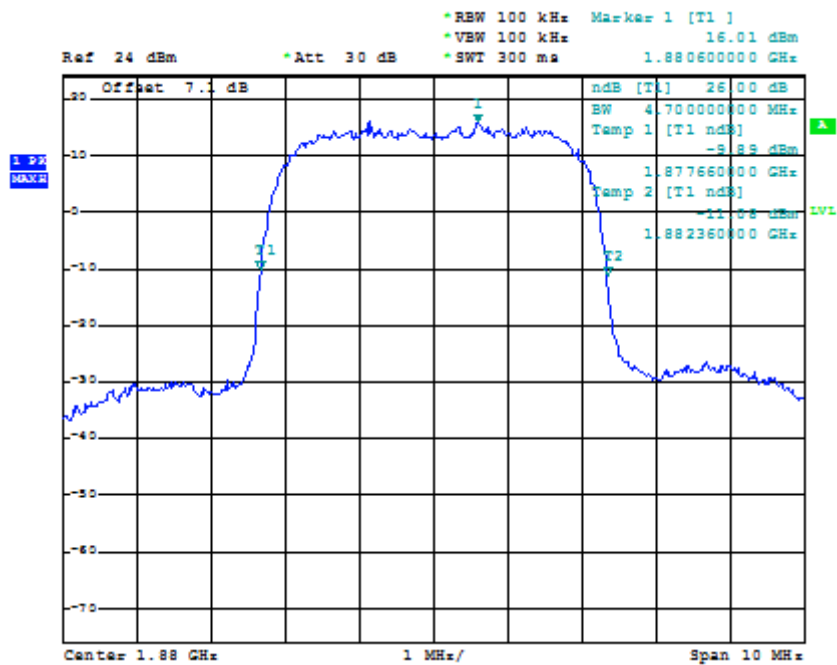
26dB Bandwidth Plot on Channel 9400
