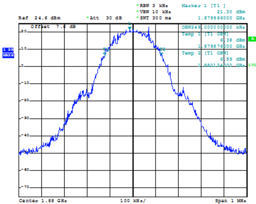
26dB Bandwidth Plot on Channel 661
