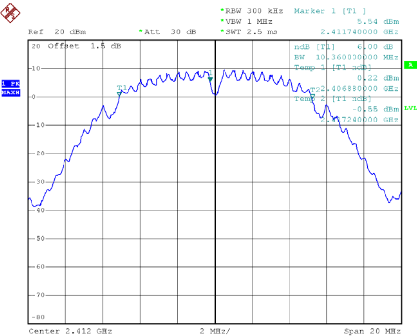
Mode 1 : 6 dB Bandwidth Plot on 802.11b Channel 01
