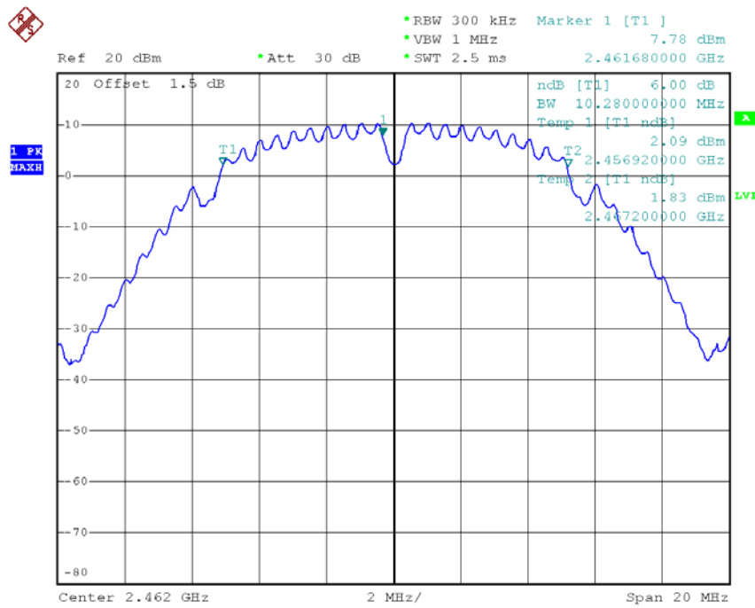
Mode 3 : 6 dB Bandwidth Plot on 802.11b Channel 11
