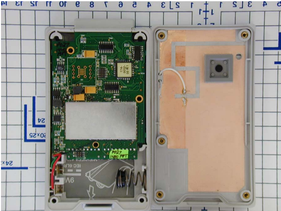
Interior View of 600 MHz ECG
