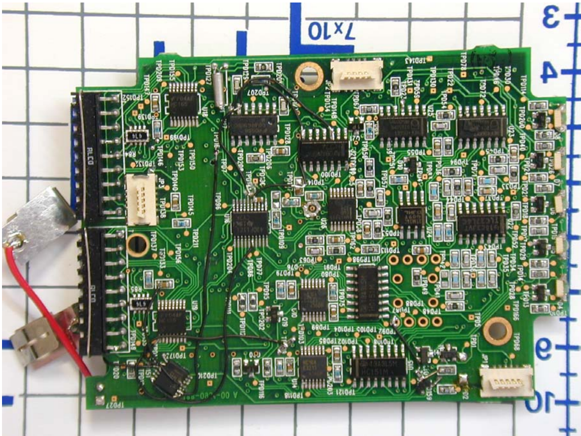
Transmitter Board Top View
