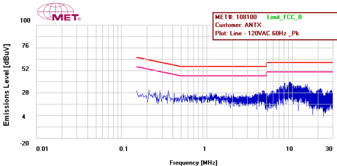
Figure 12: § 15.207(a) Conducted Emissions Limits, Line, Peak Scan
