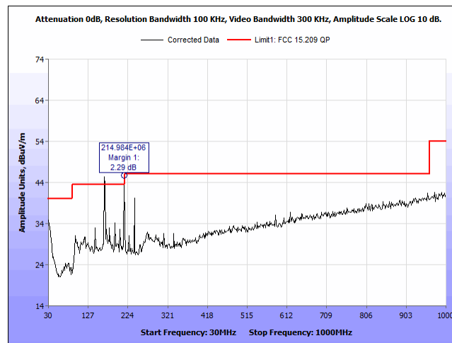
Figure 40: § 15.209 Radiated Spurious Emissions, 30-1000 MHz, 2440 MHz, Vertical, Peak Scan
