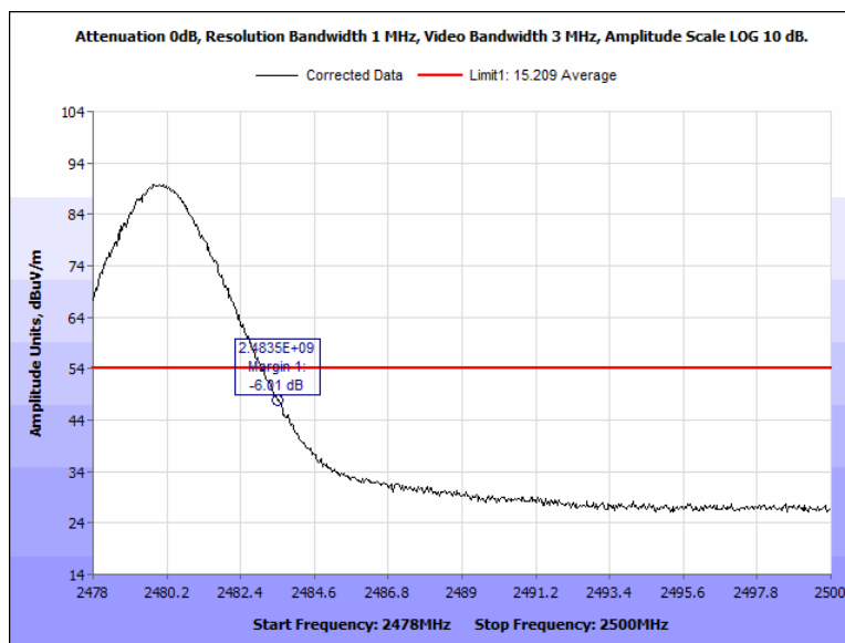
Figure 71: § 15.209 Radiated Spurious Emissions, Radiated Restricted Band Edge, 2480 MHz, Average, Vertical
