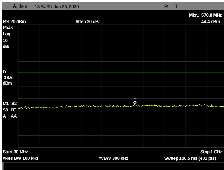
Figure 89: § 15.247(d) Spurious Emissions in Non-restricted Bands, 30-1000 MHz, 2480 MHz, 2 Mbps
