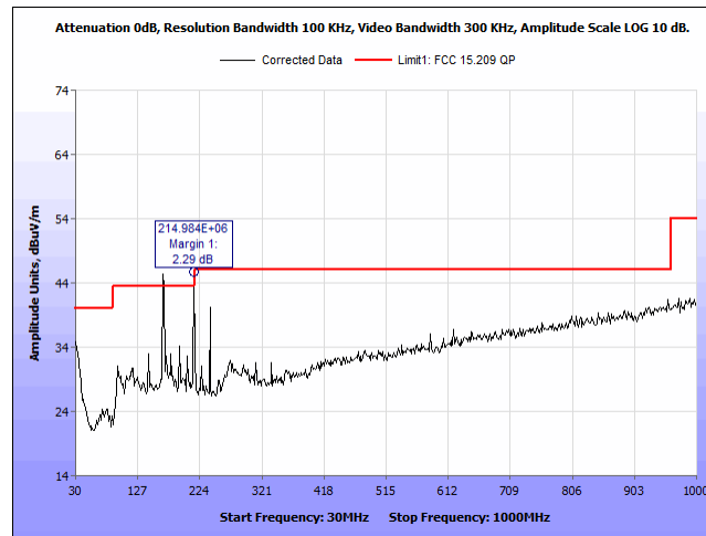
Figure 39: § 15.209 Radiated Spurious Emissions, 30-1000 MHz, 2440 MHz, Horizontal, Peak Scan
