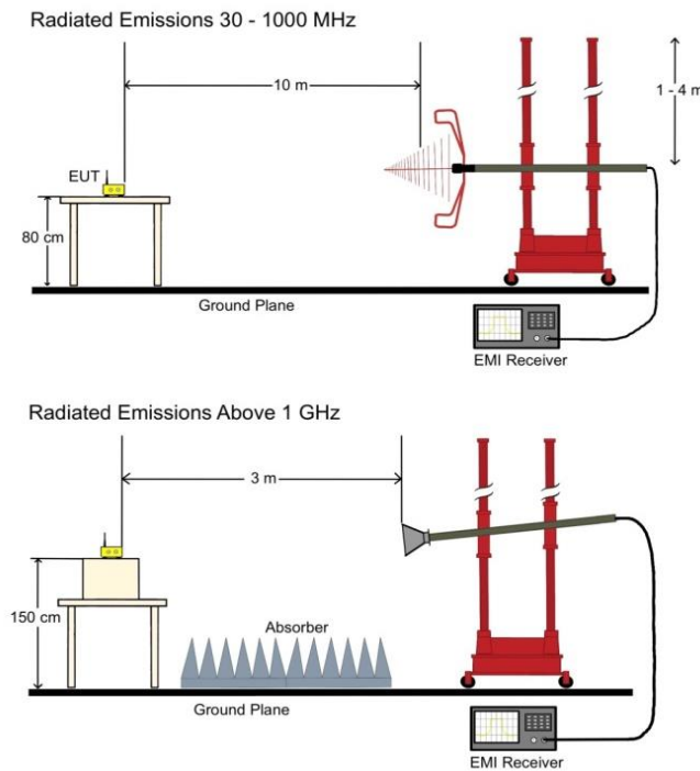
Figure 34: Radiated Emissions Test Setup
