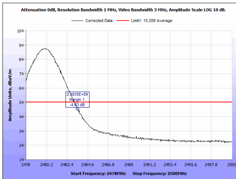
Figure 70: § 15.209 Radiated Spurious Emissions, Radiated Restricted Band Edge, 2480 MHz, Average, Horizontal
