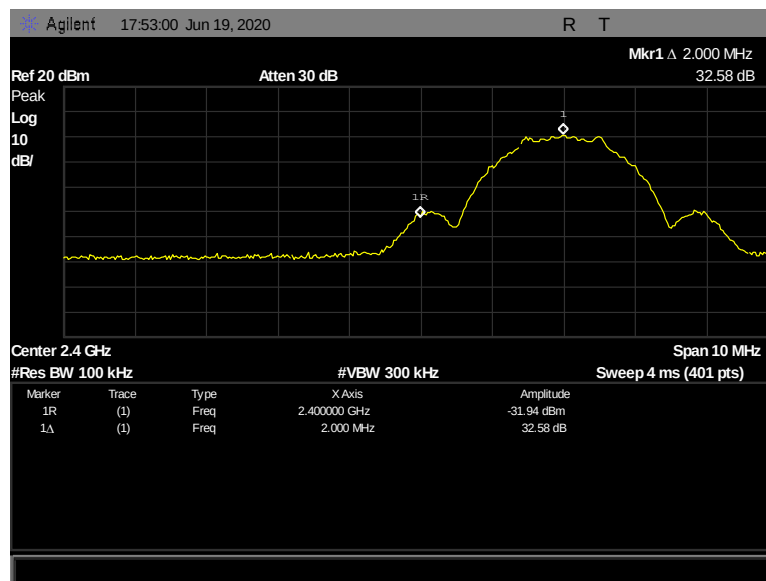
Figure 77: § 15.247(d) Spurious Emissions in Non-restricted Bands, 2402 MHz, 2 Mbps
