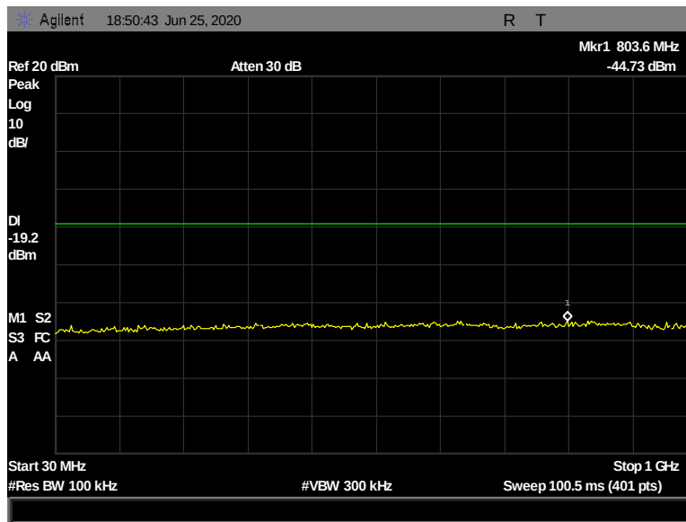
Figure 85: § 15.247(d) Spurious Emissions in Non-restricted Bands, 30-1000 MHz, 2402 MHz, 2 Mbps
