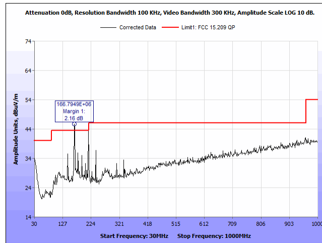
Figure 43: § 15.209 Radiated Spurious Emissions, 30-1000 MHz, 2480 MHz, Vertical, Peak Scan
