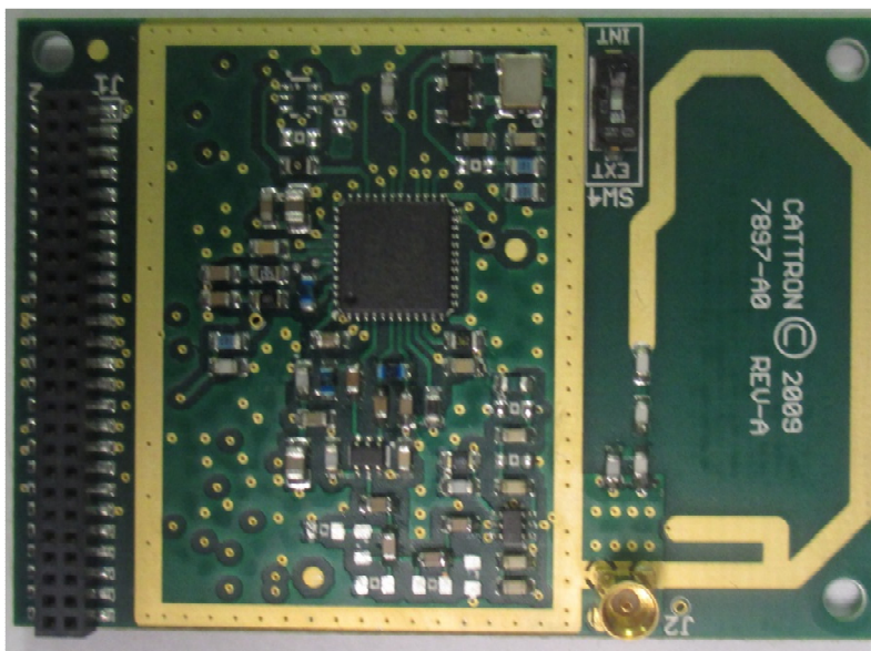
ADL450MHz 78970 TRX TOP without shielding
