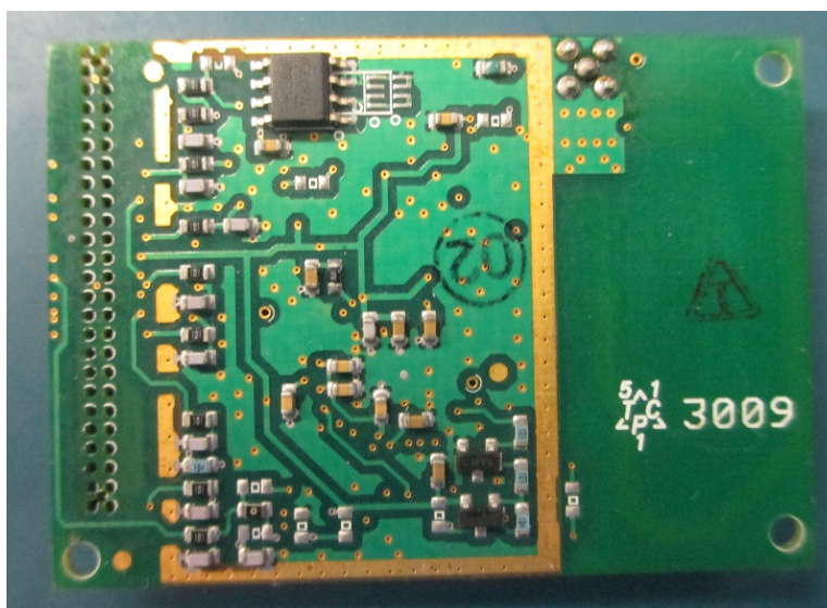
ADL450MHz 78970 TRX BOTTOM without shielding
