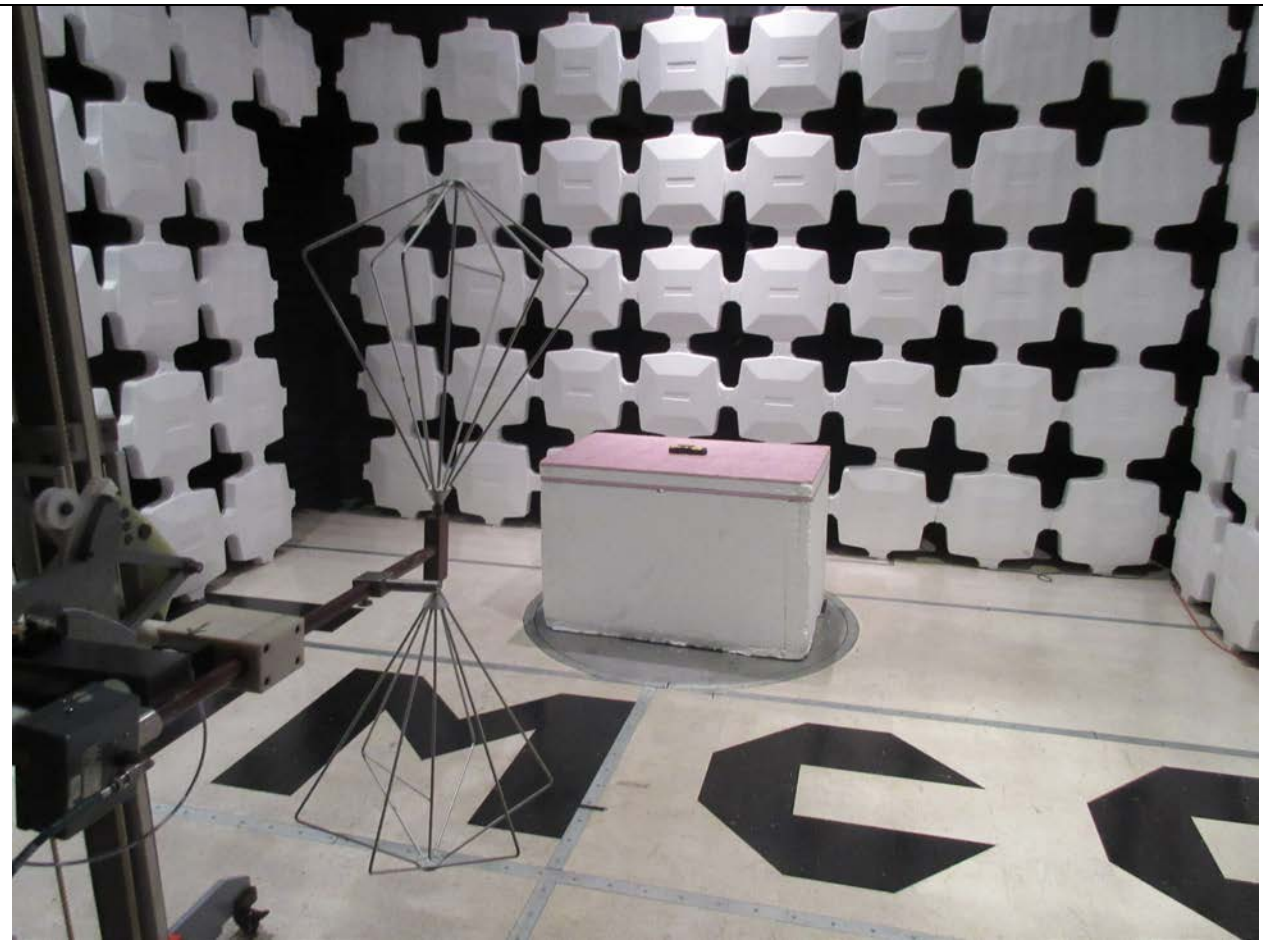
Radiated Emissions Final Setup
