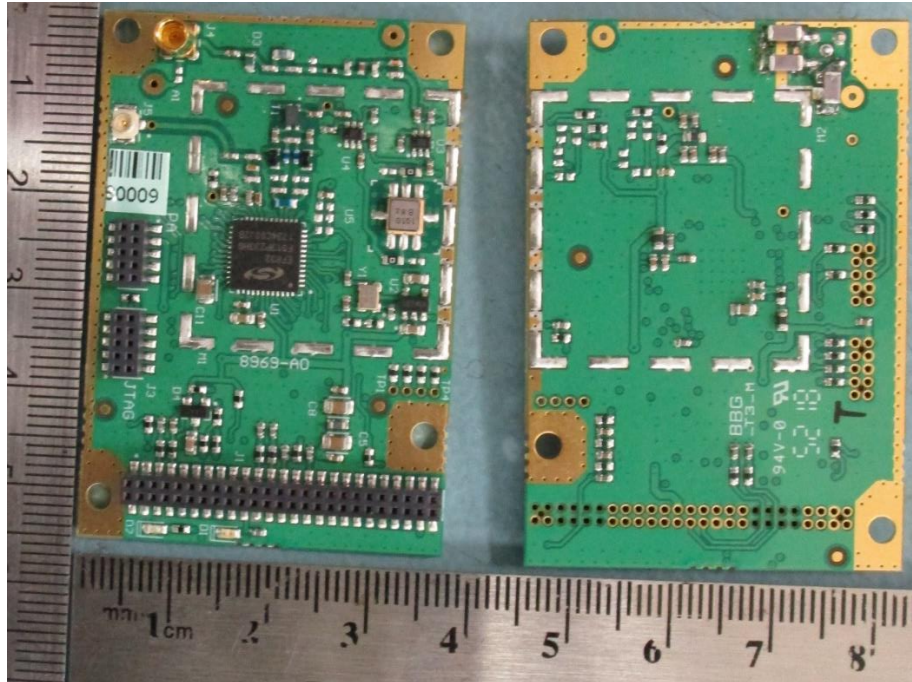
TOP and BOTTOM view without Shielding
