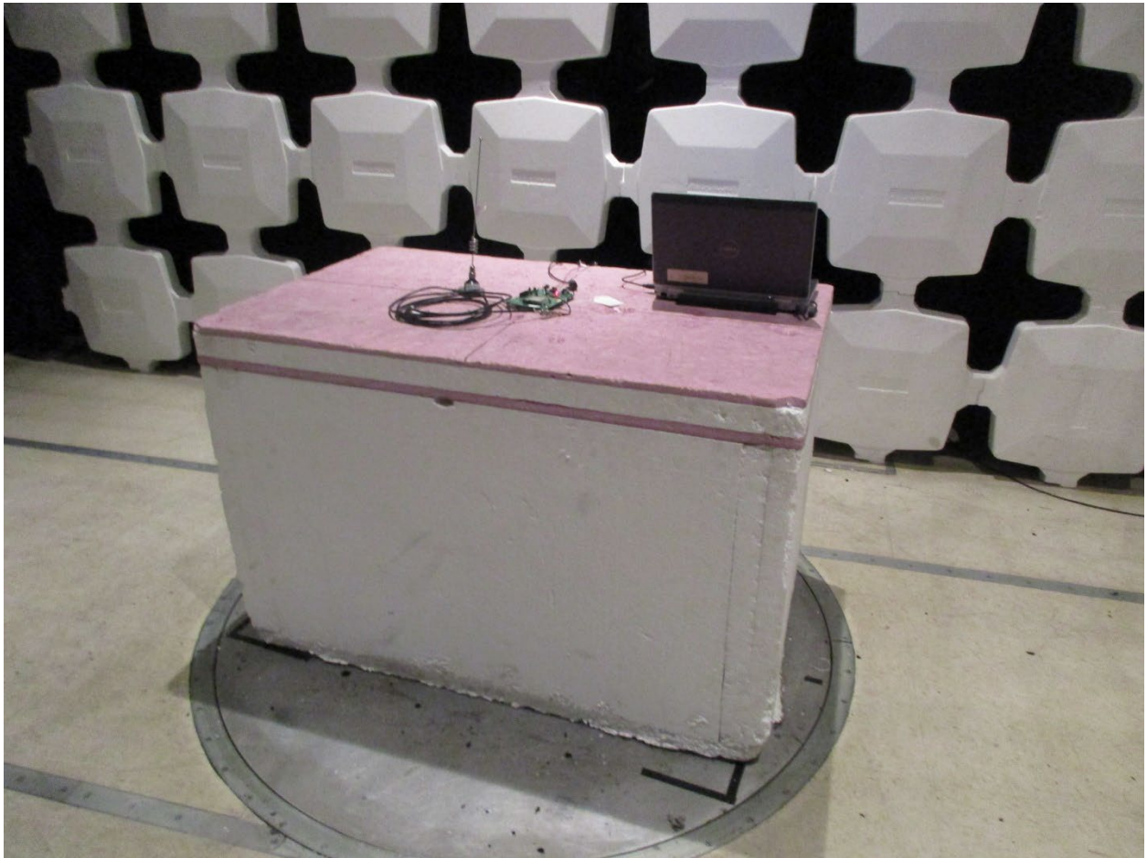
Radiated Testing, Table Setup #3
