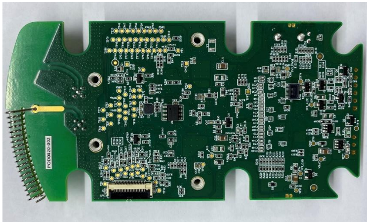
OCU Inside Front View
