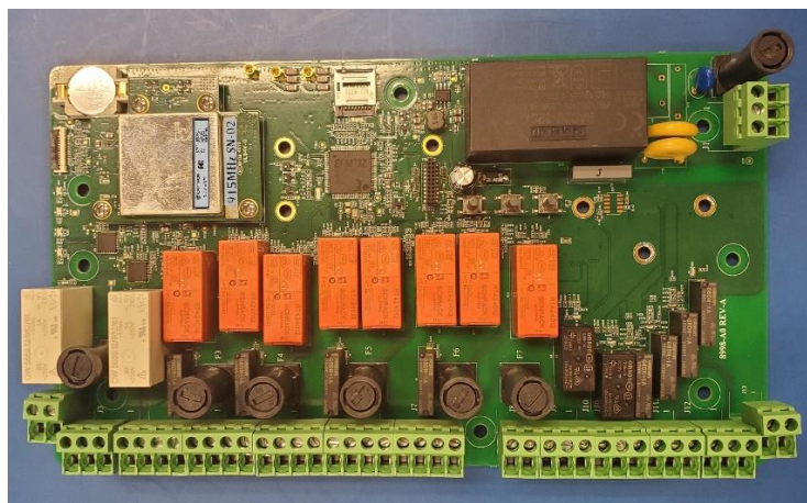
MCU inside view
