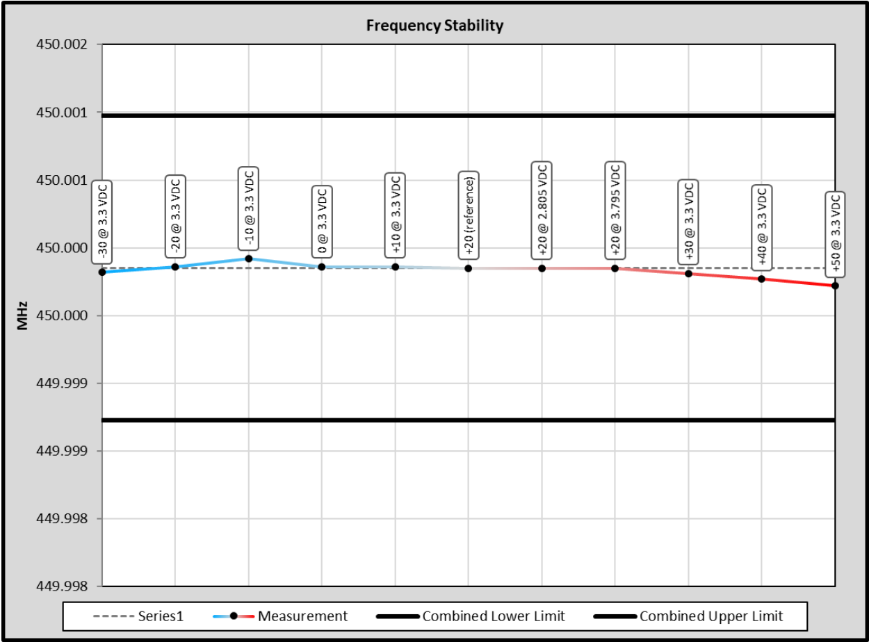
Test Data: 450-470 MHz Band Plot
