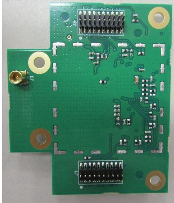
BOTTOM View
