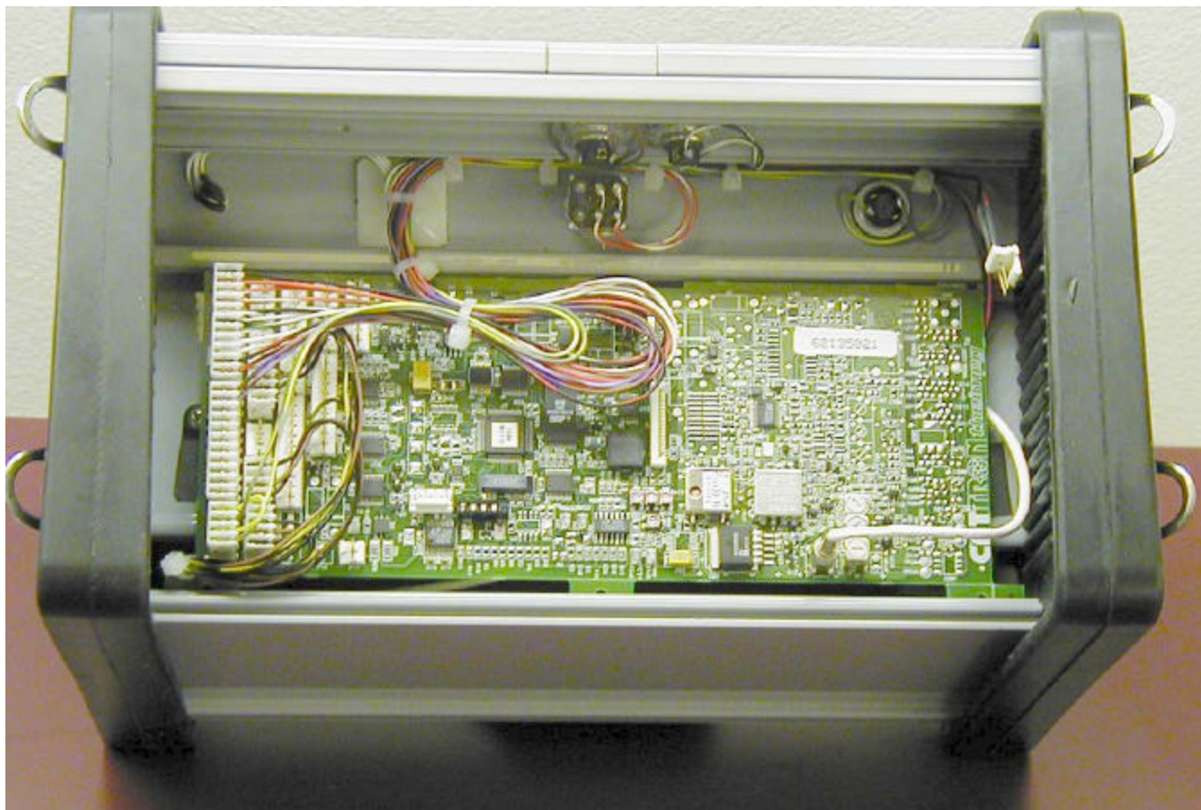
Enclosure Open (Battery Compartment Removed)
