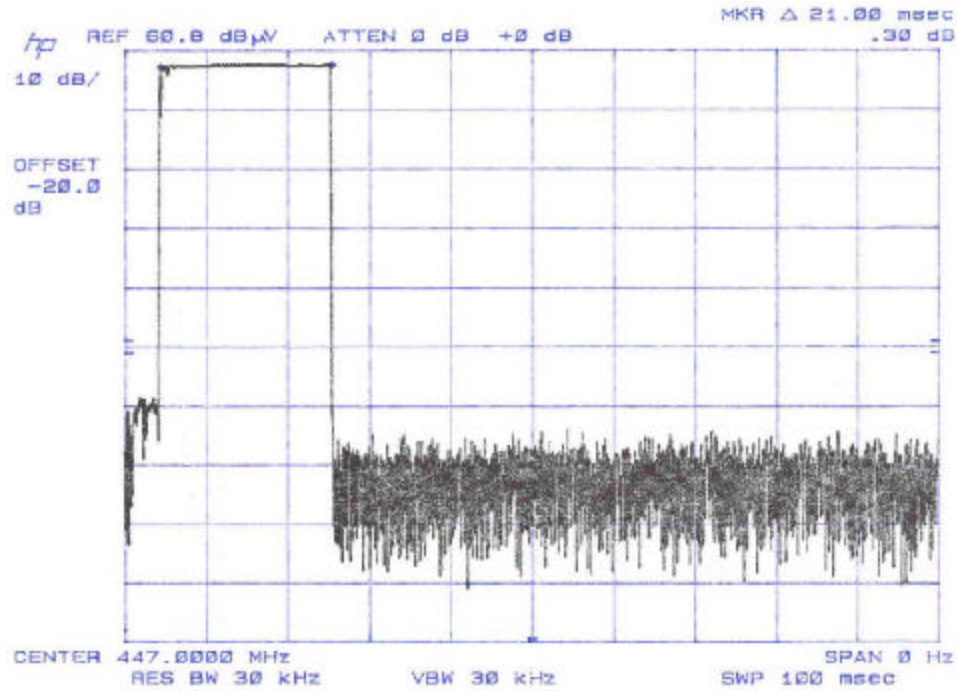
Figure 1. Channel 0 Duty Cycle, Pulse Width (100ms)
