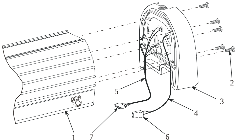
Figure 4-3. Top Endcap Sub-assembly, removal and replacement
