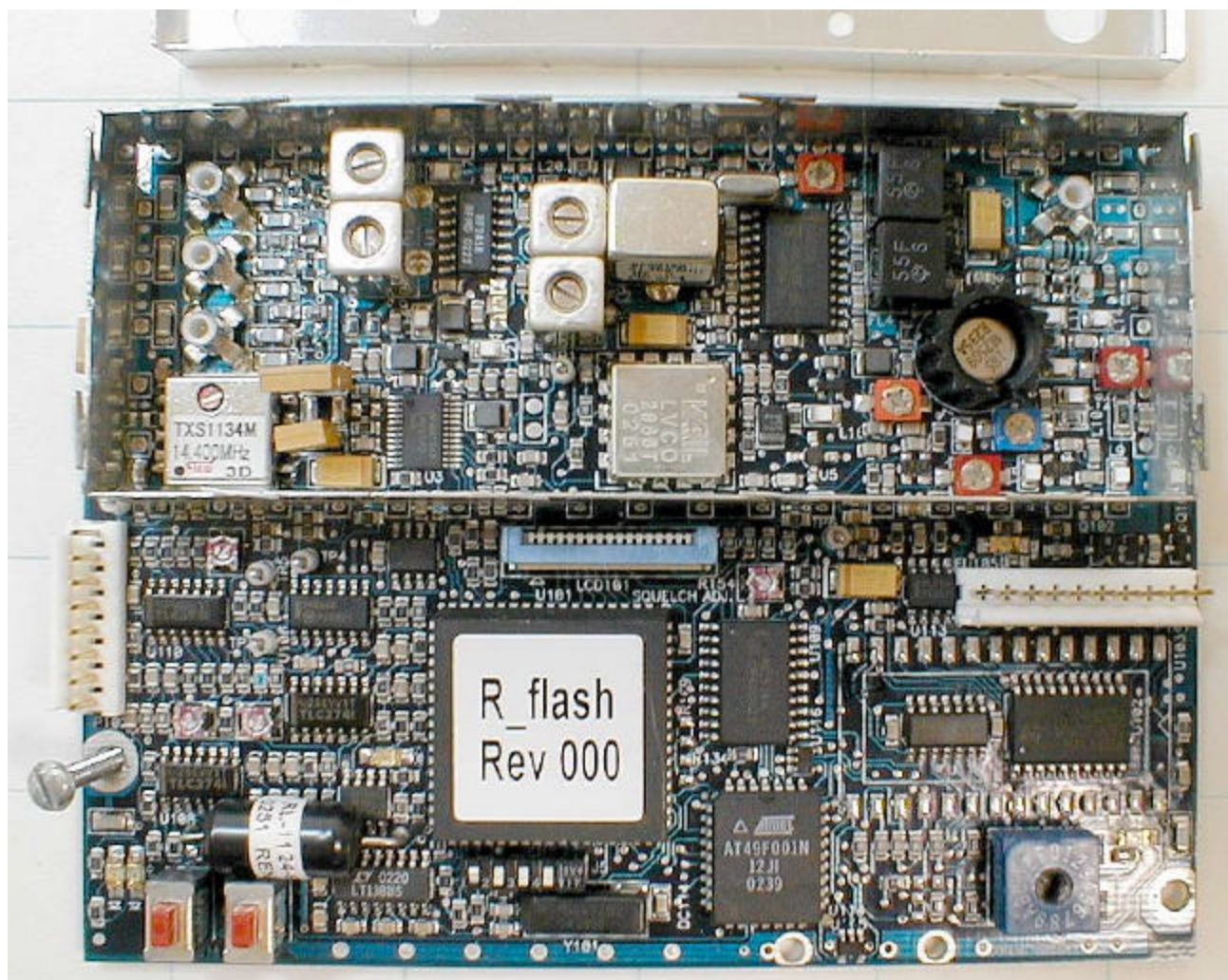
R3A Board Top View, Shield and LCD Readout Removed
