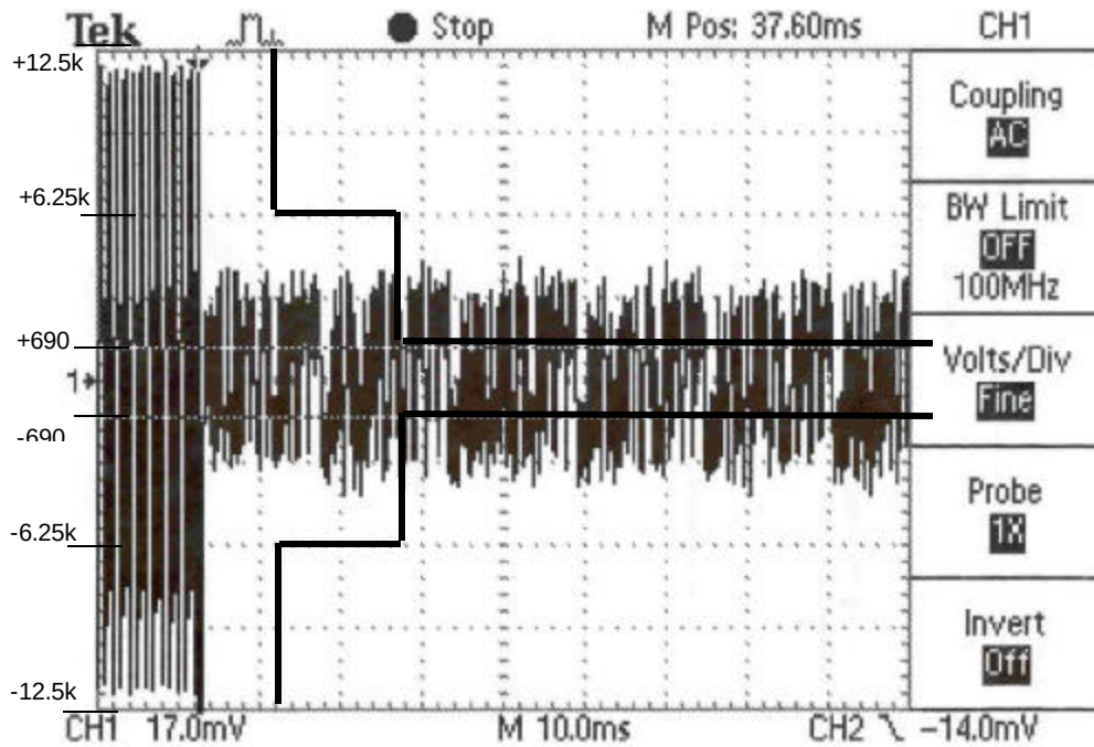
Figure 27. Transient Frequency Response: 460MHz ON Time
