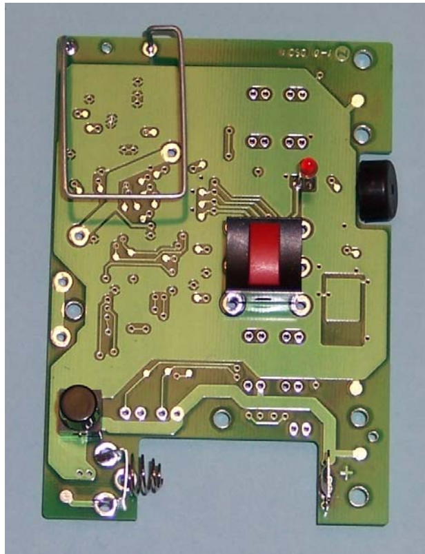
Bottom View of PCB
