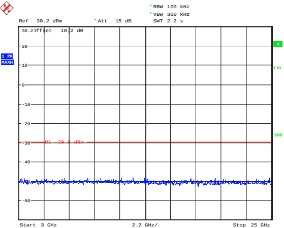
Low Channel 3 GHz – 25 GHz
