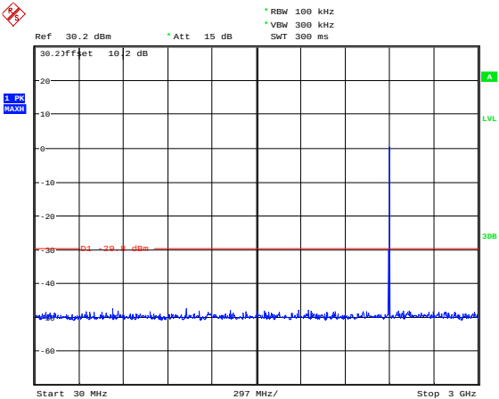
Low Channel 30 MHz – 3 GHz
