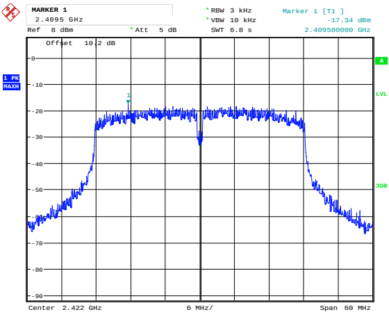
Low Channel 2422 MHz
