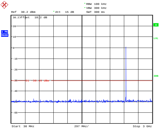
Middle Channel 30 MHz – 3 GHz
