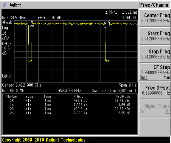
802.11n20 mode
