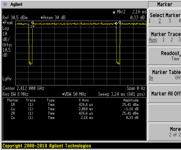
802.11g mode
