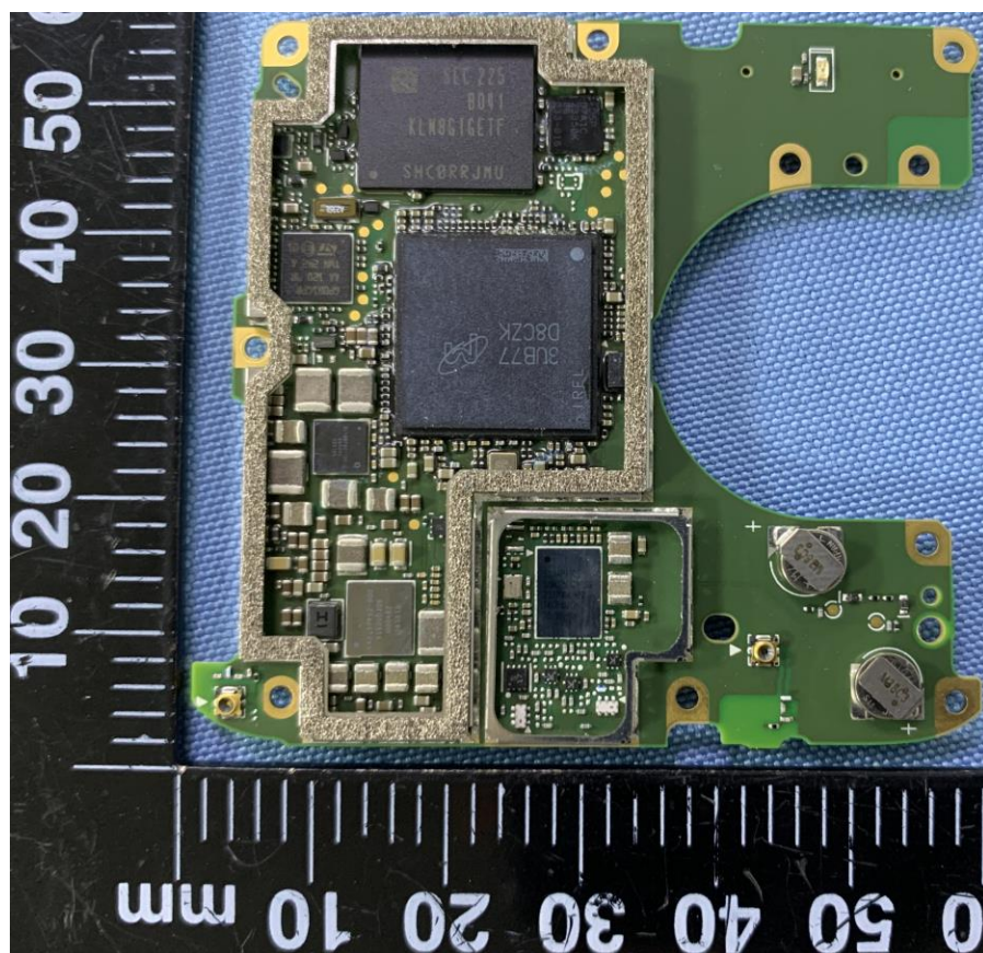
340-32177-000, ASSY, PCBA, MAIN PEBBLES -Front with shield removed, CPPB1
