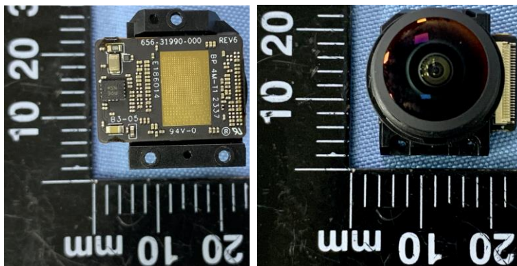
340-31995-000, PCBA, REAR,IMU, SENSOR BOARD, PEBBLES, CPPB1
