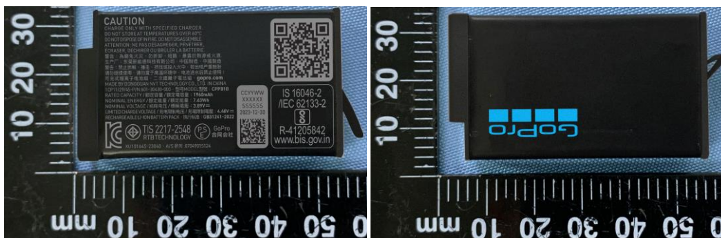
Li-ion Battery Pack, CPPB1B
