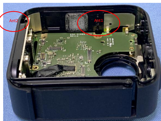
BT/WIFI antenna location, CPPB1
