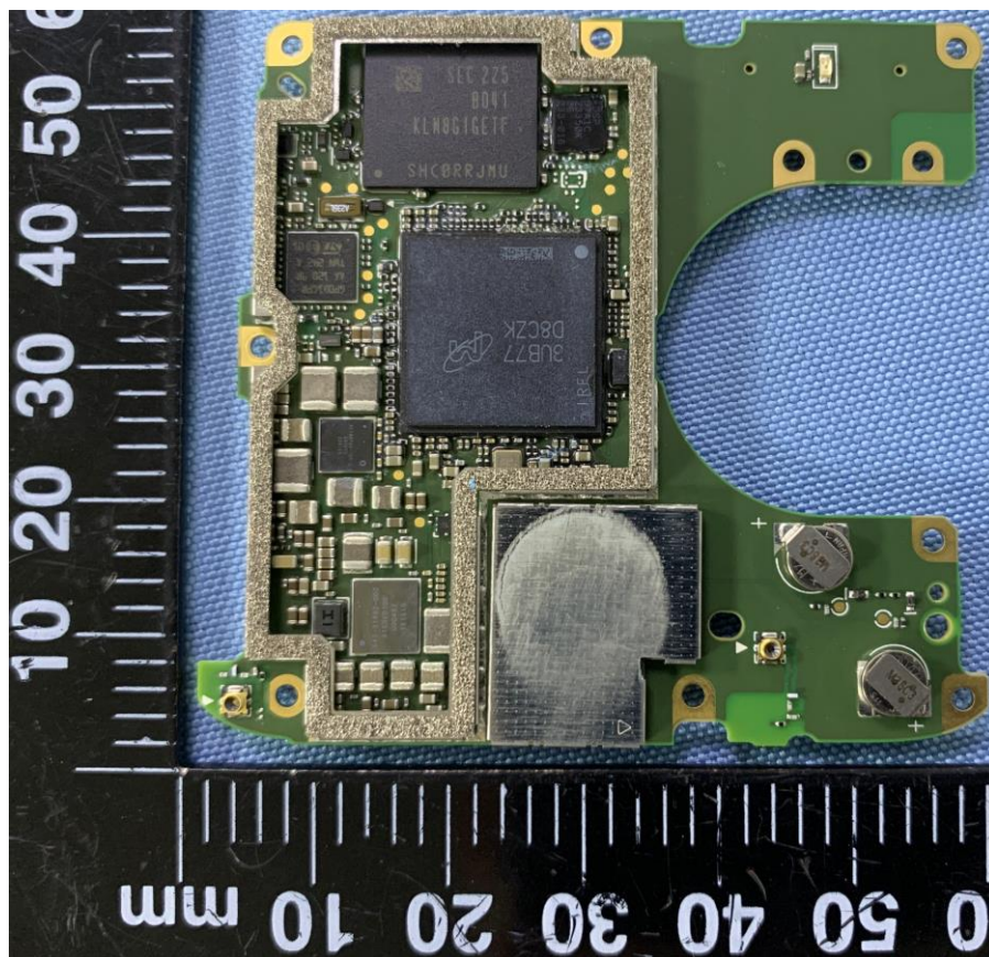
340-32177-000, ASSY, PCBA, MAIN PEBBLES -Front with shield, CPPB1
