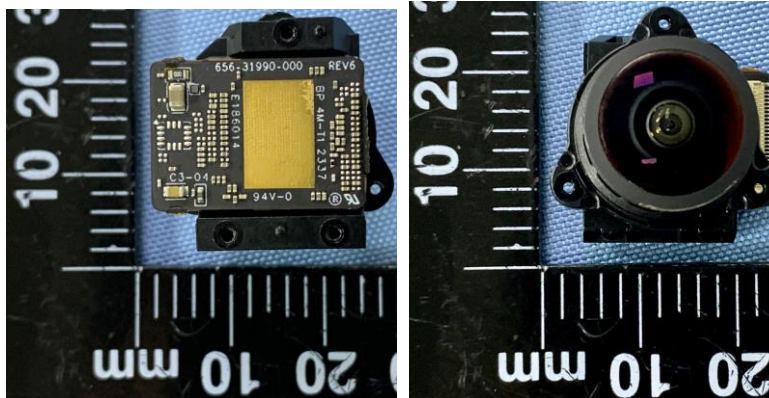
340-31996-000, PCBA, FRONT, NO IMU, SENSOR BOARD, PEBBLES, CPPB1
