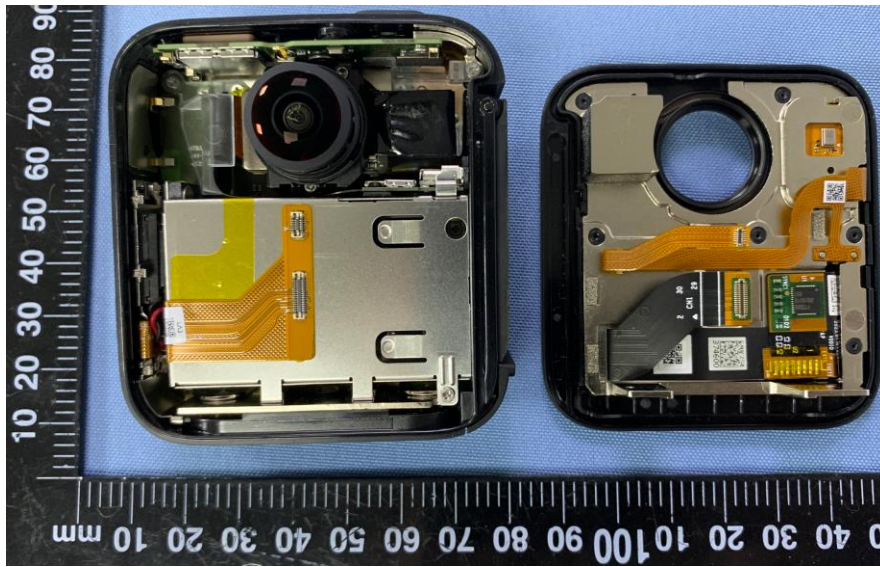
Rear cover removed, CPPB1
