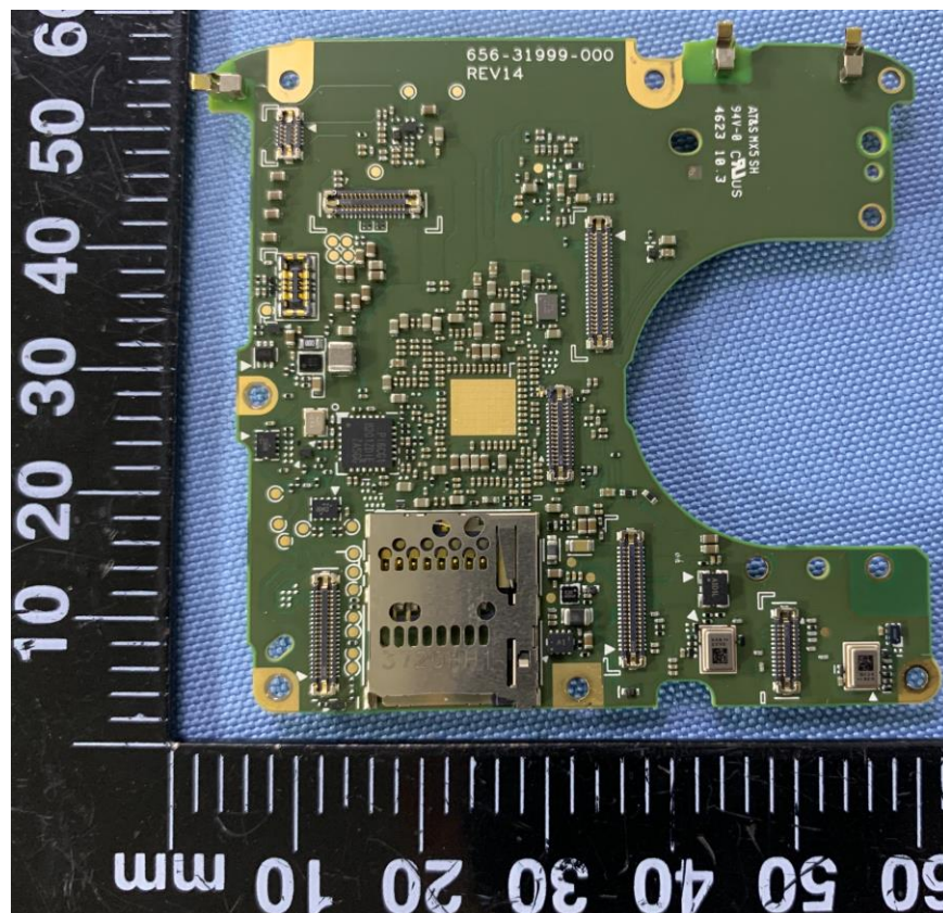
340-32177-000, ASSY, PCBA, MAIN PEBBLES -Rear, CPPB1
