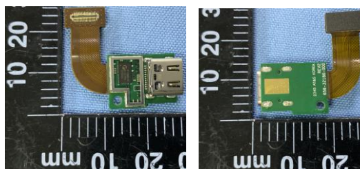
340-32192-000, ASSY, PCBA, RFPC, USBC, PEBBLES, CPPB1
