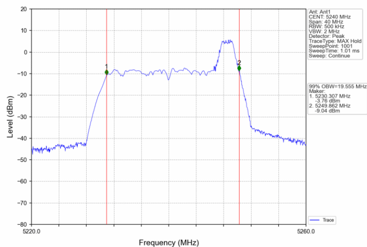
802.11ax(HEW20)_HCH_5240MHz_RU52_40_Ant1_NTNV
