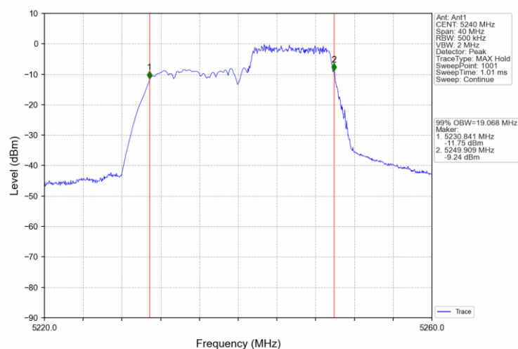
802.11ax(HEW20)_HCH_5240MHz_RU242_61_Ant1_NTNV
