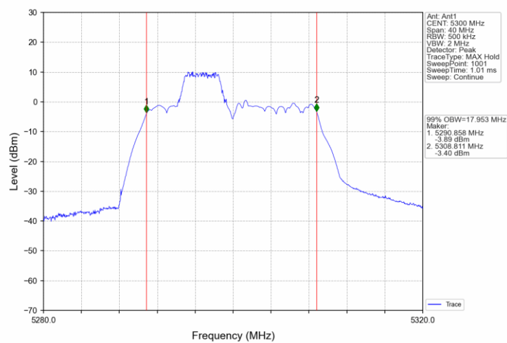
802.11ax(HEW20) MCH 5300MHz RU106_53 Ant1 NTNv
