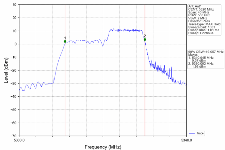
802.11ax(HEW20)_HCH_5320MHz_RU242_61_Ant1_NTNV
