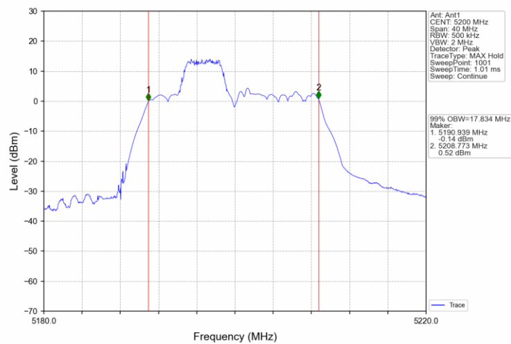
802.11ax(HEW20) MCH 5200MHz RU106_53 Ant1 NTNv
