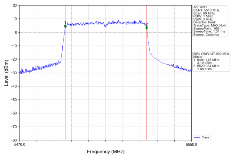
802.11ac(VHT40)_LCH_5510MHz_Ant1_NTNV
