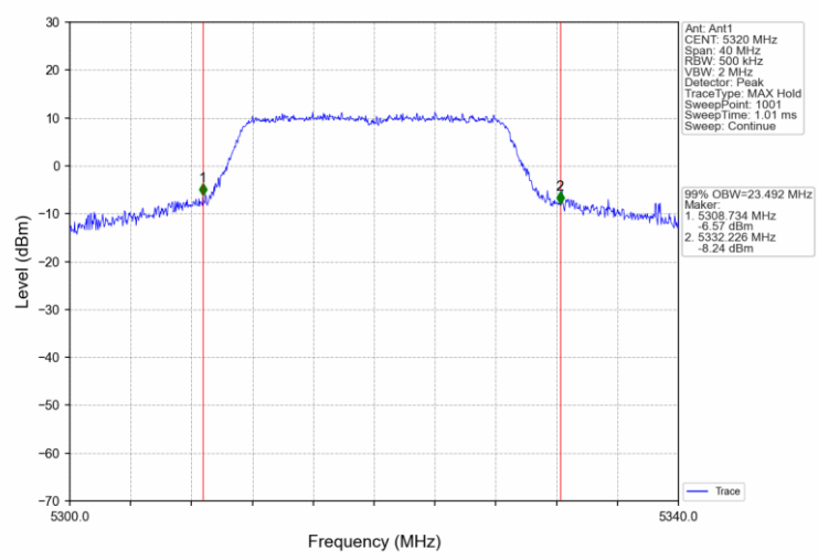
802.11ac(VHT20)_HCH_5320MHz_Ant1_NTNV
