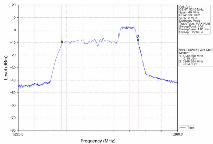
802.11ax(HEW20)_HCH_5240MHz_RU106_54_Ant1_NTNV
