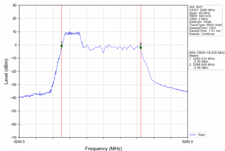
802.11ax(HEW20) LCH 5260MHz RU106_53 Ant1 NTNv
