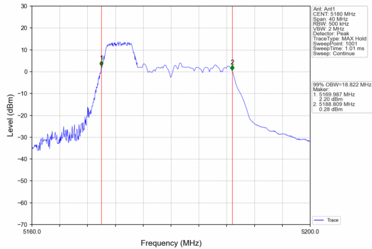
802.11ax(HEW20) LCH 5180MHz RU106_53 Ant1 NTNv
