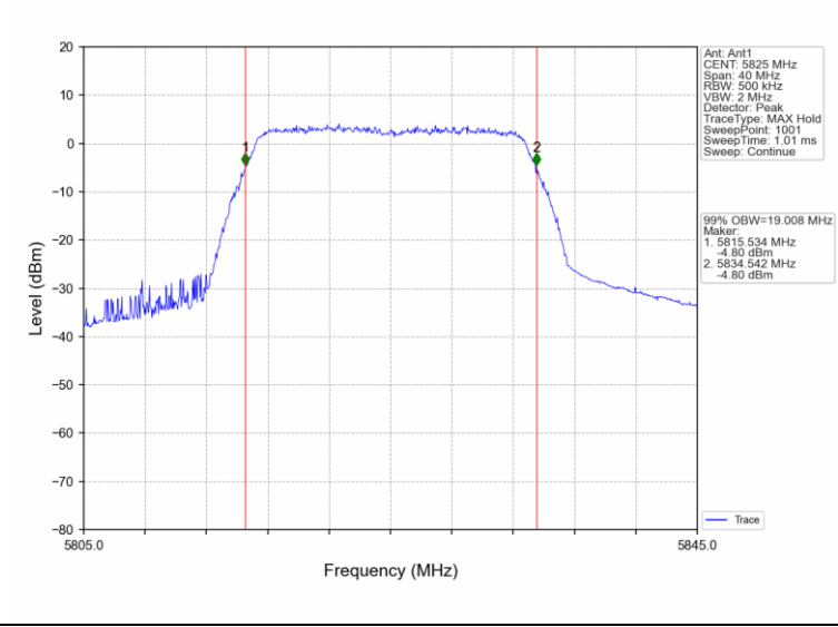
802.11ac(VHT20)_HCH_5825MHz_Ant1_NTNV
