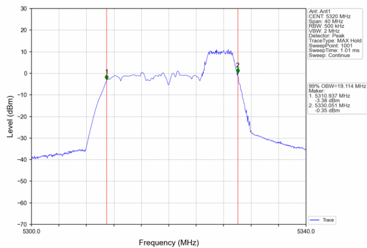
802.11ax(HEW20)_HCH_5320MHz_RU106_54_Ant1_NTNV
