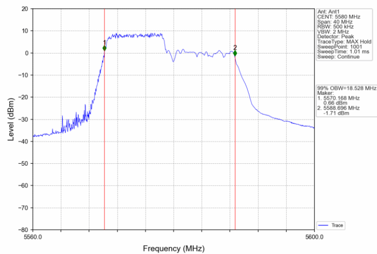
802.11ax(HEW20) MCH 5580MHz RU242_61 Ant1 NTNv
