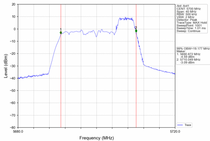
802.11ax(HEW20)_HCH_5700MHz_RU106_54_Ant1_NTNV
