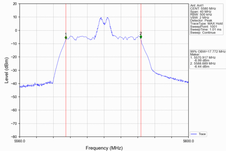
802.11ax(HEW20) MCH 5580MHz RU52_38 Ant1 NTNv
