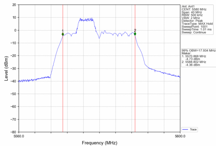
802.11ax(HEW20) MCH 5580MHz RU106_53 Ant1 NTNv
