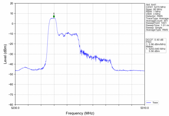
802.11ax(HEW40)_LCH_5270MHz_RU106_53_Ant1_NTNV
